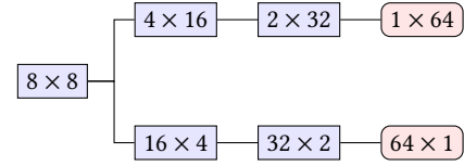
Figure 6: Recursive intersection hierarchy
