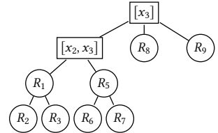
Figure 9. A compatible free-connex join tree for Q_4 .
