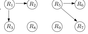
Fig. 16. Query-update graph of Q_4 .
