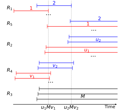
Figure 12. A reduction from an OuMv instance to a \sigma -sequence for Q_{\text{path}} , where \sigma(\{e_1\}) and \sigma(\{e_4\}) are not insertion-only.
