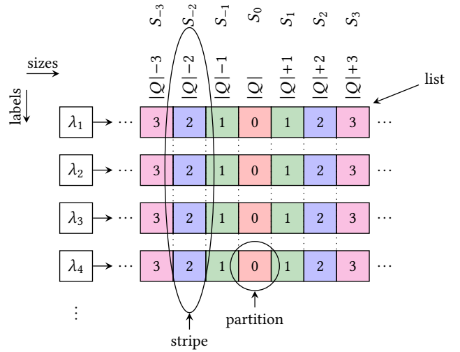
Figure 4: Stripes and partitions w.r.t. query Q .
