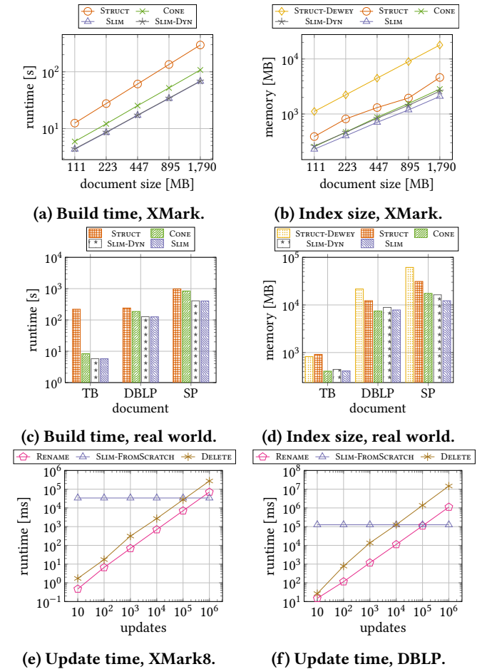
Figure 12: Build time, index size, and update time.
