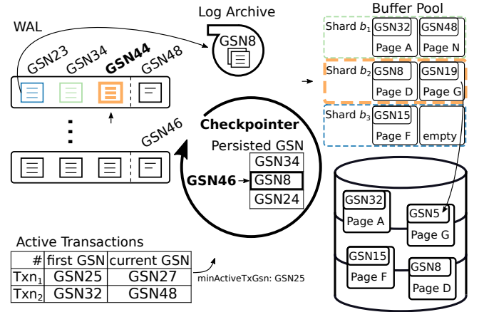
Figure 5: Checkpointing example. The frequency of checkpoint increments is coupled to WAL volume.
