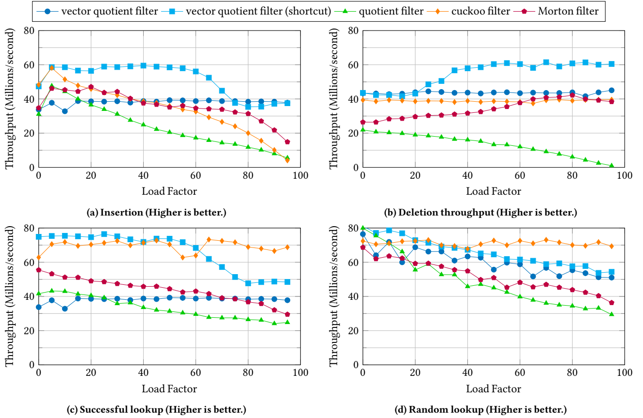
Figure 5: Insertion, deletion, and lookup performance of different filters in L3 cache. The vector quotient filter with shortcut refers to the optimization described in Section 6.2. All filters were configured with a target false-positive rate of 2^{-8} , as described in Table 2.
