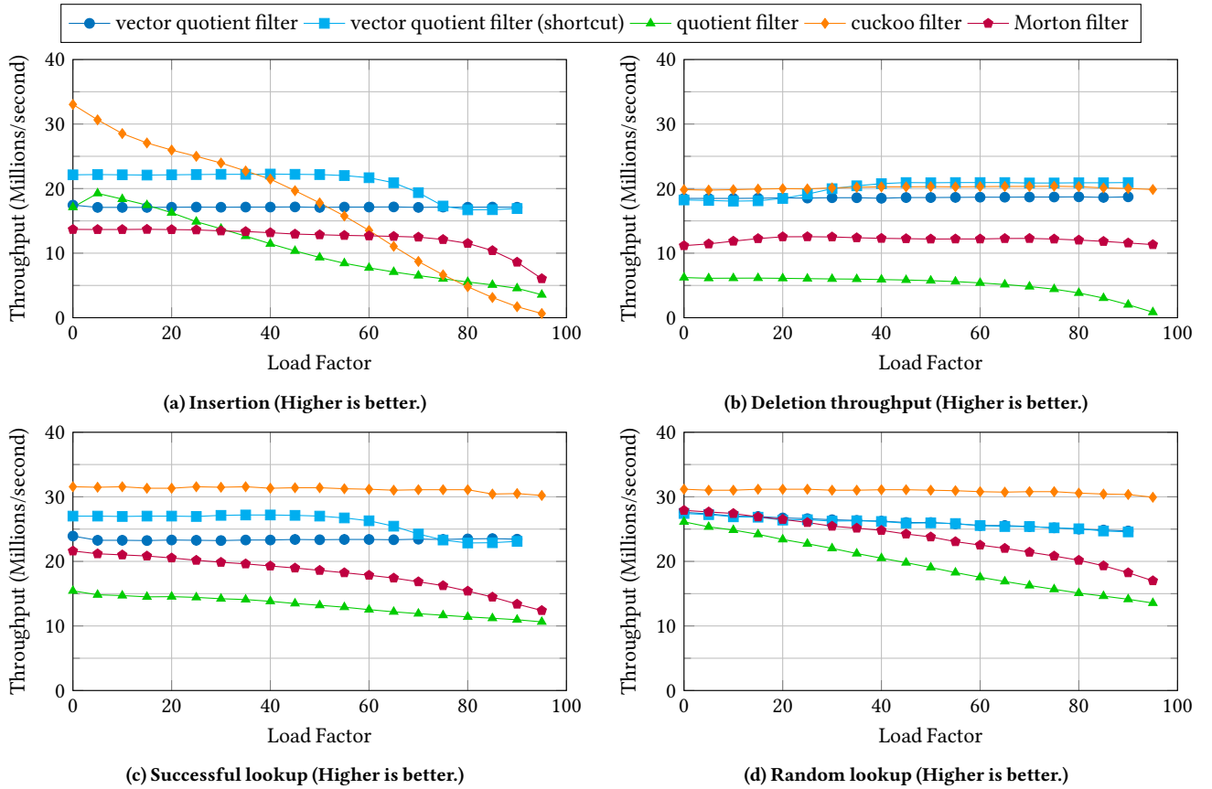
Figure 4: Insertion, deletion, and lookup performance of different filters in RAM. All filters were configured with a target false-positive rate of 2^{-8} , as described in Table 2. Shortcut refers to the optimization described in Section 6.2. Note that in Figure 4d, the lines for the vector quotient filters with and without the shortcut optimization nearly coincide. The vector quotient filter is shown with throughput only up to 90% because it reaches full capacity at 93%.
