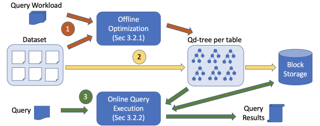
Figure 4: (1) In offline optimization, MTO produces a layout (a qd-tree per table) given a dataset and query workload. (2) MTO assigns records to blocks and stores them. (3) In online query execution, MTO skips blocks based on the layout.
