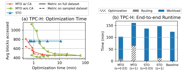
Figure 13: (a) MTO and STO can decrease optimization time by using sampling. Cardinality adjustment (CA) helps MTO mitigate performance degradation. (b) MTO achieves the lowest end-to-end runtime when optimized with a 3% data sample.
