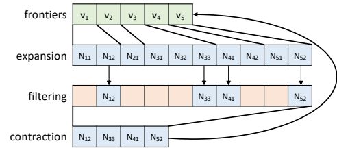
Figure 2: Parallel graph processing computational pipeline.
