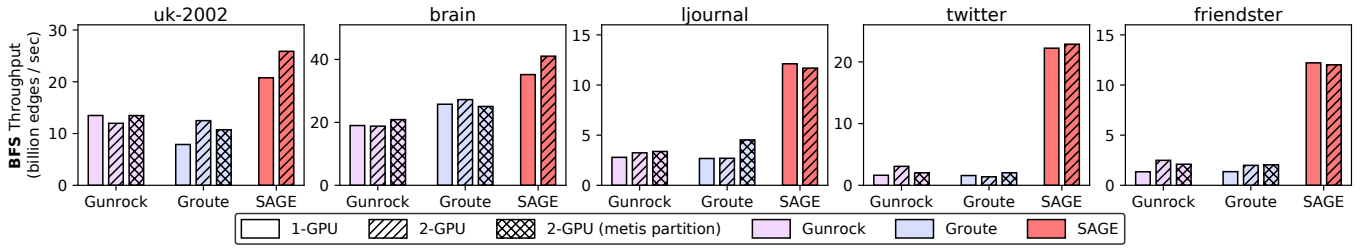
Figure 9: Comparison between SAGE and multi-GPU baselines.
