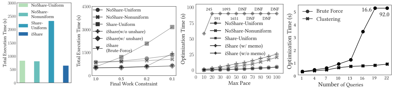
Figure 13: Manually tuned paces Figure 14: Tests for decomposition algorithm Figure 15: Overhead of end-to-end optimization Figure 16: Optimization overhead of Clustering algorithm
