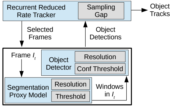
Figure 2: OTIF execution pipeline architecture. The tracker selects which frames to process. To detect objects in each sampled frame, the segmentation proxy model determines which windows of the frame may contain objects, and the detector runs in those windows. Parameters selected by the tuner are shown in grey.
