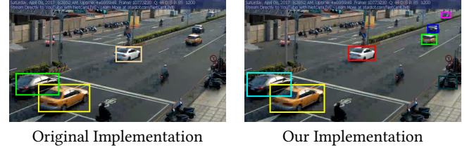
Figure 8: The original BlazeIt implementation detects cars in the authors’ Taipei video with unreasonably poor accuracy. On the left, we show detections taken directly from files published by the authors. Our implementation improves over the original in accuracy and delivers similar speed.
