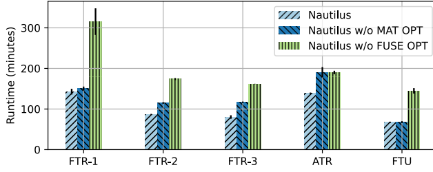
Figure 8: Model selection time with and without MAT and FUSE optimizations.
