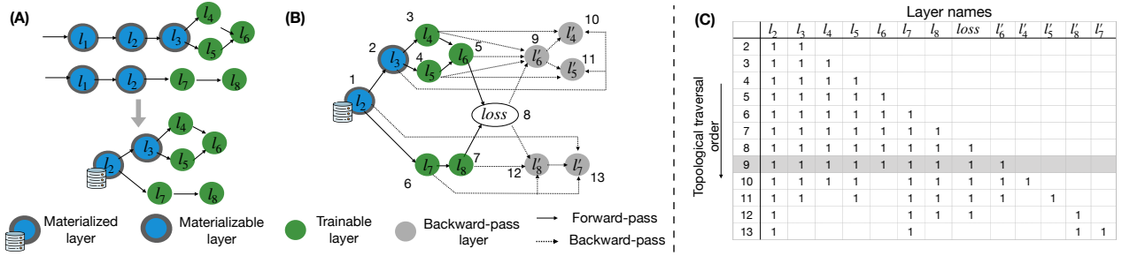
Figure 5: (A) A candidate partition containing two source models and the corresponding optimal reuse-plan model. (B) Augmenting reuse plan model with nodes to represent the backward-pass of training. (C) Topological traversal-based live tensor analysis for the model graph shown in (B).
