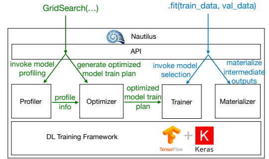
Figure 3: High-level architecture of NAUTILUS and the interactions between system components. fit(...) method is called for every model selection cycle.
