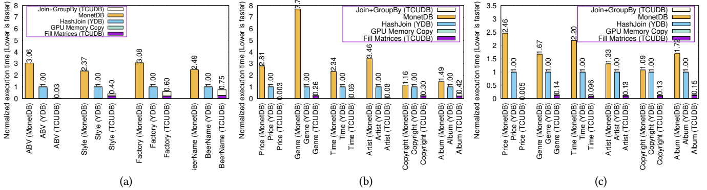
Figure 11: The relative runtime of the EM-blocking queries on TCUBD using the default deepmatcher datasets (a) BeerAdvocate (b) iTunes-Amazon and (c) scaled iTunes-Amazon, compared to MonetDB and YDB running the same query as the baseline.
