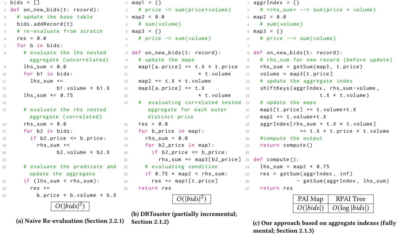
Figure 2: Code corresponding to different execution strategies for the query in Example 2.2.
