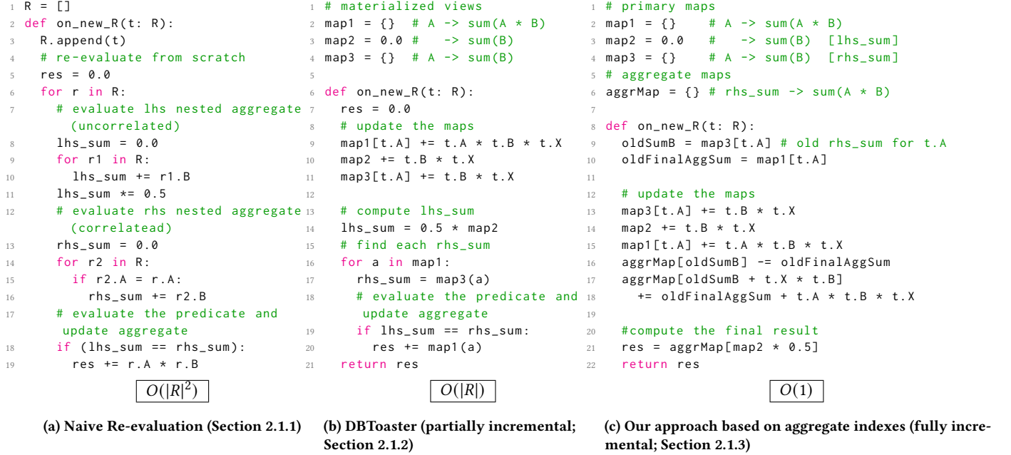
Figure 1: Code corresponding to different execution strategies for the query in Example 2.1 (assuming O(1) hash map access).
