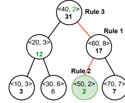
Figure 3: An example run of the \text{getSum}(50) . The red lines show the traversal path, and the values in green color contribute to the final answer which is 12+2+2 . Each node shows \langle \text{key}, \text{value} \rangle and the subtree sum.
