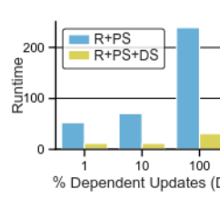
Figure 16: Dependent Updates
