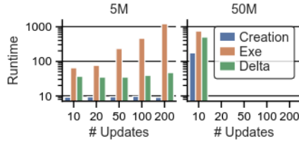
Figure 12: Breakdown Naïve
