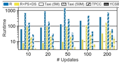
Figure 15: Optimization
