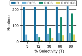
Figure 17: Affected Data
