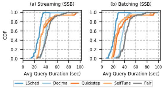
Figure 9: Comparing LSched with other scheduling baselines under streaming and batched (SSB) queries.
