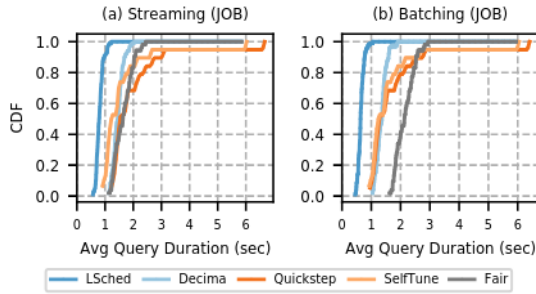
Figure 10: Comparing LSched with other scheduling baselines under streaming and batched (JOB) queries.
