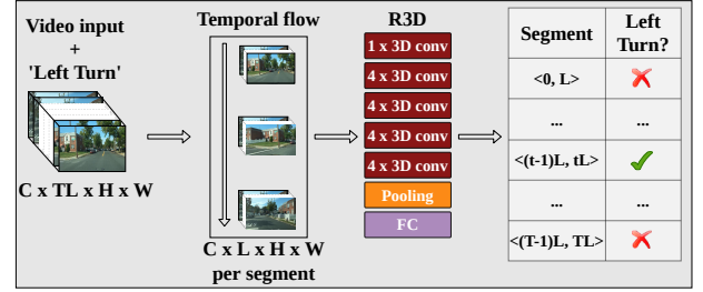
Figure 4: In ZEUS-SLIDING, the input video of T \times L frames is divided into T segments of L frames each. Each segment is then processed by the R3D network to generate binary class labels to determine the presence/absence of action.
