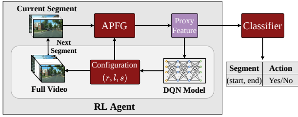
Figure 5: Architecture of QUERY EXECUTOR in ZEUS – The QUERY EXECUTOR uses a deep RL agent to process action queries. It takes as input the PROXYFEATURE generated by the APFG, to output a CONFIGURATION, which is used to construct the next input segment. The PROXYFEATURE is also processed by a classifier to predict the presence of action in the current segment.
