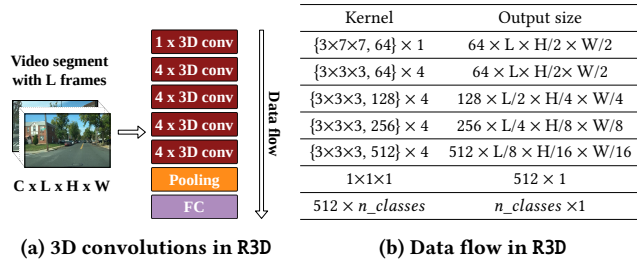
Figure 3: The R3D network consists of 17 3D convolutional layers followed by adaptive average pooling and fully-connected layers. The input to the network is a video segment of length L frames. In successive 3D convolutional operations, the input is reduced to eventually get a 512 dimensional feature vector.
