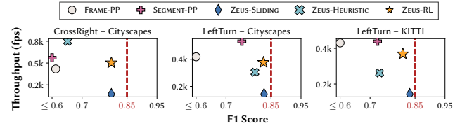
Figure 13: Domain Adaptation – Throughput and F1 score of ZEUS-RL and other baselines trained on the BDD100k dataset and evaluated on the Cityscapes and KITTI datasets.
