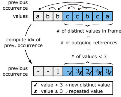
Figure 1: Computing a windowed COUNT DISTINCT by evaluating a 2-dimensional range query.
