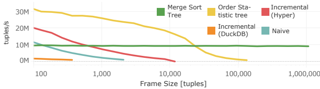
Figure 11: Throughput of a framed median for increasing frame sizes.
