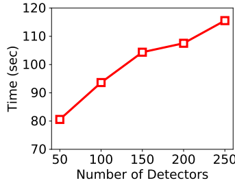
Fig. 6. Scalability on the Number of Detectors
