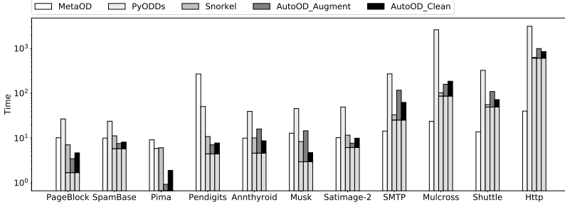
Fig. 5. Runtime Evaluation
