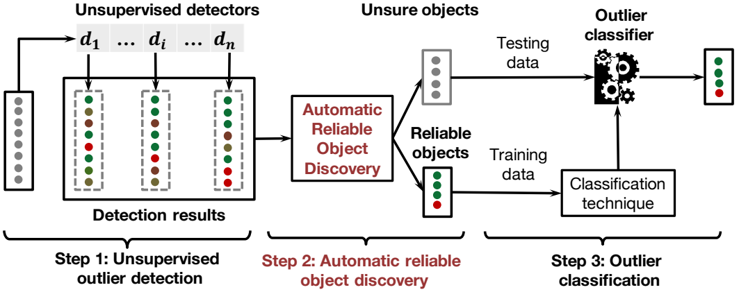
Fig. 1. AutoOD Framework
