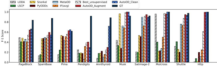
Fig. 4. Effectiveness Evaluation of All Methods on Ten Benchmark Data Sets using F-1 Metric
