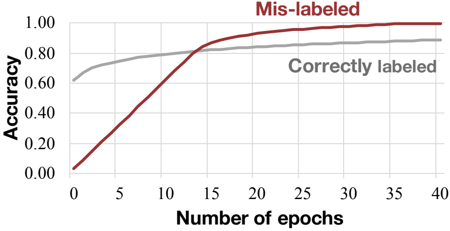
Fig. 3. Observation: Evolution of Training Accuracy for Mislabeled and Correctly Labeled Samples.
