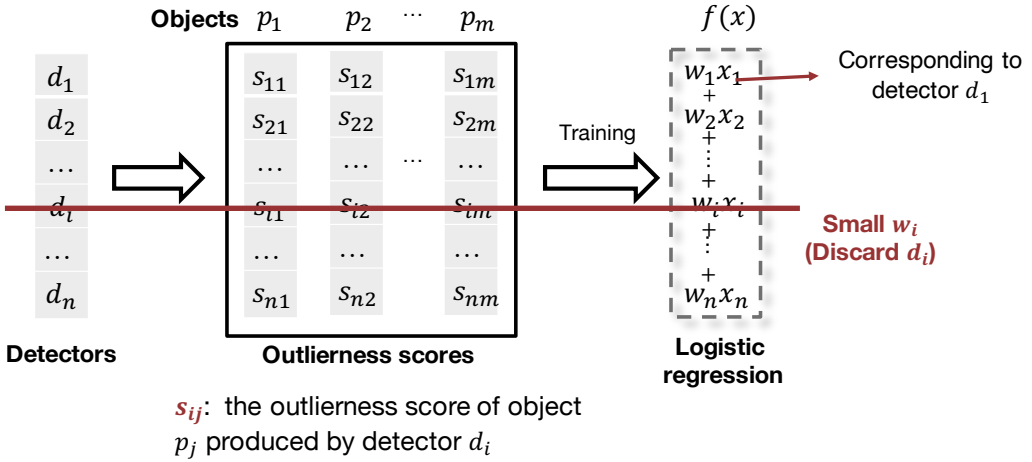
Fig. 2. AutoOD-Augment: Prune Poor Detectors
