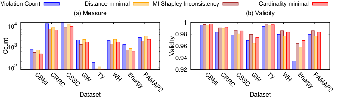
Fig. 21. Validity by various inconsistency measures
