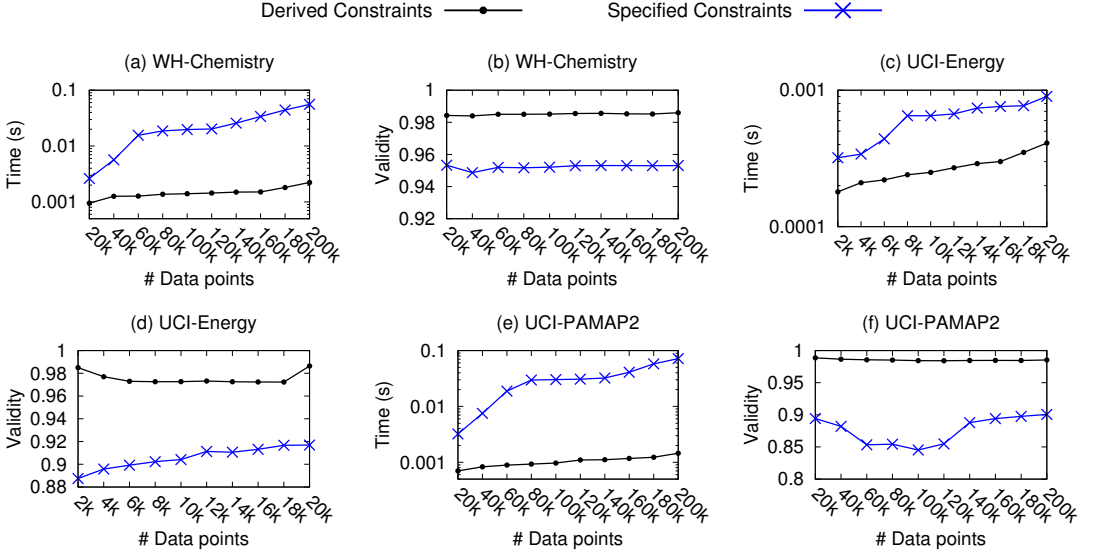
Fig. 10. Evaluation on derived constraints
