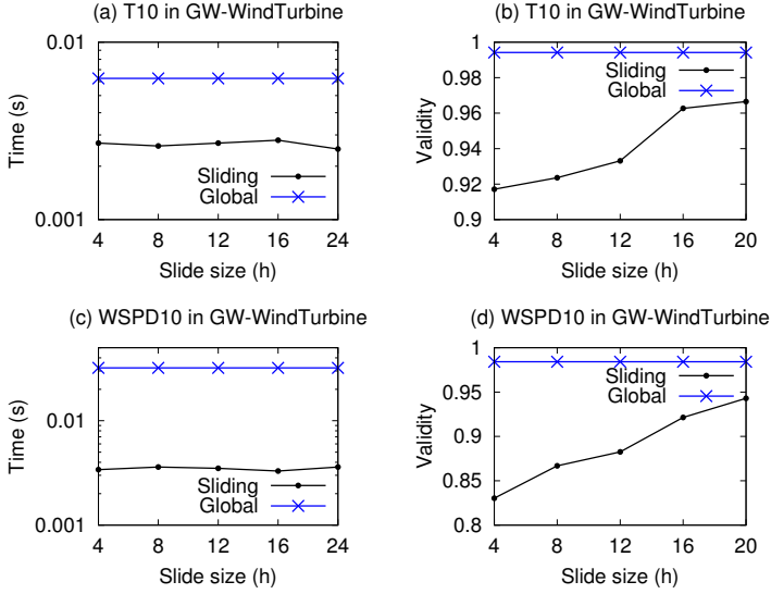
Fig. 14. Evaluation on constraints in sliding windows
