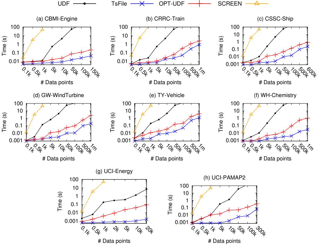
Fig. 7. Validity computation under different data sizes
