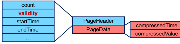
Fig. 6. Page in TsFile
