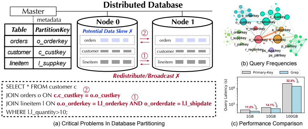
Fig. 1. Example Database Partitioning on TPC-H Schema.
