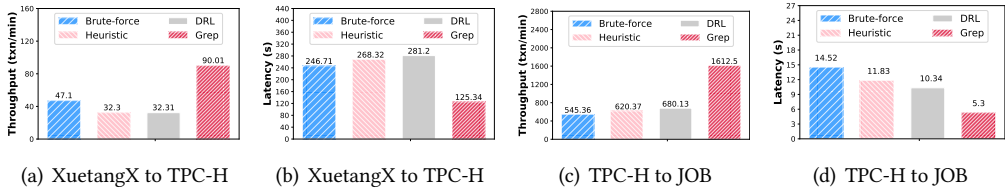
Fig. 9. Dataset Adaptability on Postgres-XL.
