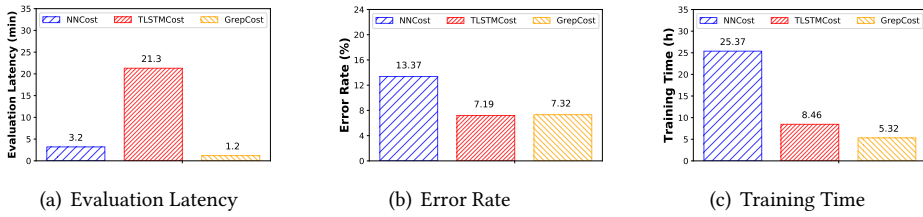
Fig. 7. Performance Evaluation of TPC-H workloads.
