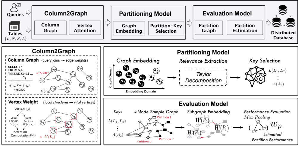
Fig. 2. The Grep Overview.
