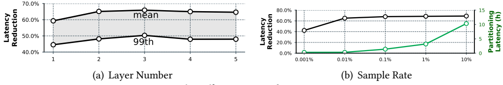
Fig. 8. The Effectiveness of Hyper-Parameters.
