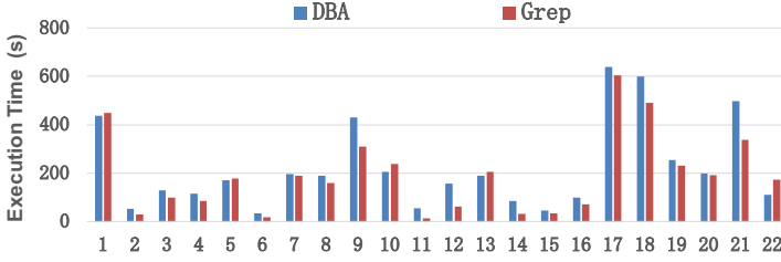
Fig. 6. Performance of TPC-H Queries (on Commercial Database). Grep gains 14.2% reduction in total.
