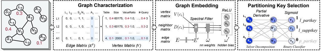
Fig. 4. Graph-based Key Selection Model.
