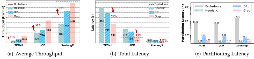
Fig. 5. Performance Comparison with Baselines.
