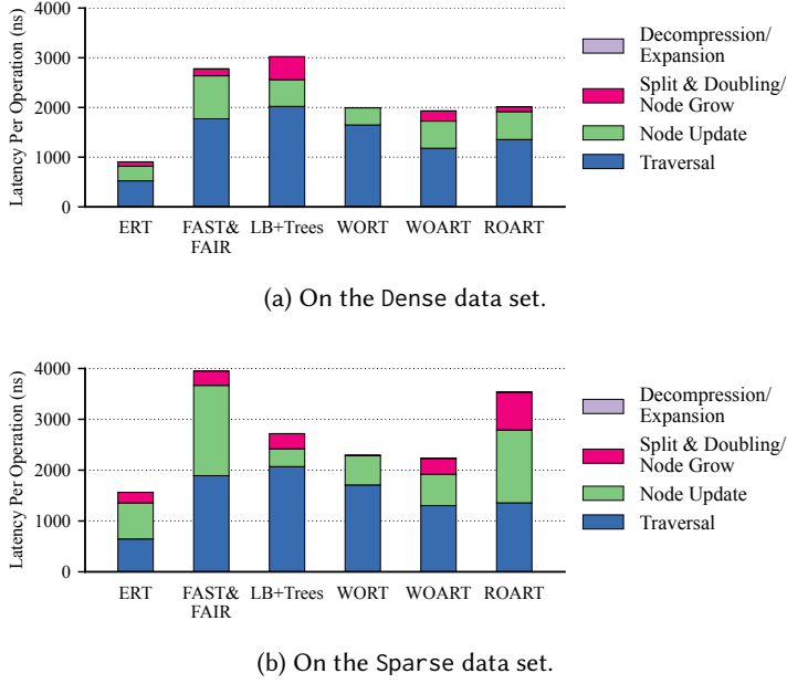
Fig. 11. Latency breakdown for insert operations.
