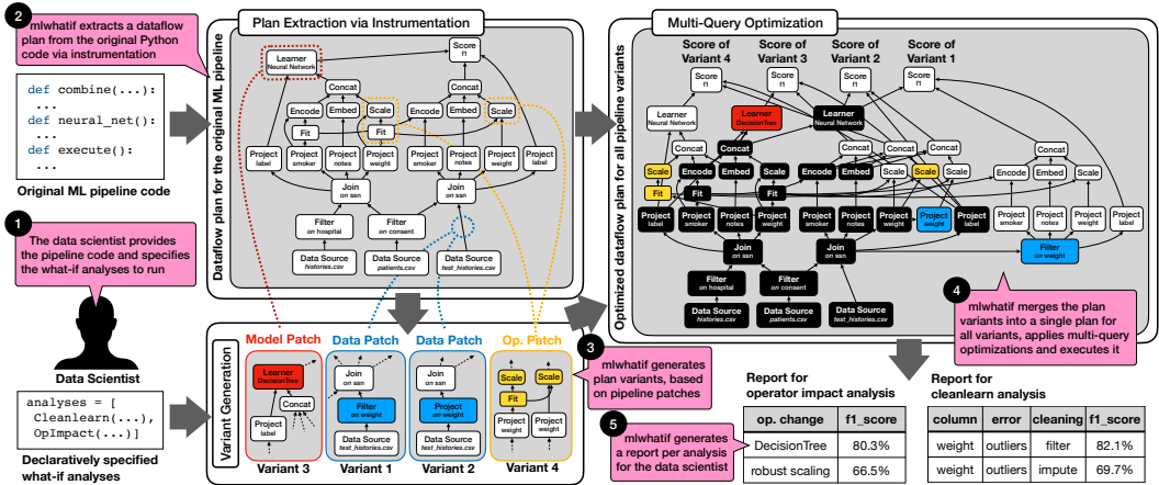
Fig. 1. Overview of mlwhatif : The data scientist provides the code for an ML pipeline (Listing 1) and declaratively specifies the what-if analyses to run on that pipeline 1 . Next, mlwhatif extracts a dataflow plan from the original pipeline via code instrumentation 2 . Based on the specified what-if analyses and the extracted plan, mlwhatif generates different pipeline variants with “pipeline patches” 3 , and merges the variants into a single joint dataflow plan. Next, mlwhatif applies various multi-query optimization rules to re-use shared intermediates (illustrated as black operators) between variants 4 . Finally, mlwhatif executes the optimized plan, and generates a report per analysis, which details the variants and their output scores 5 .
