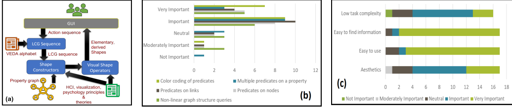
Fig. 5. (a) Overview of VEDA; (b) - (c) User survey on desirable features in Cypher GUI.
