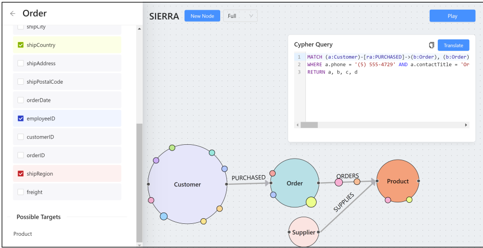
Fig. 2. The LCG abstraction of SIERRA.
