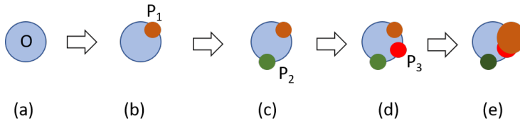
Fig. 4. Evolution of a composite circle. (a) No predicate; (b)-(d) Three predicates on three properties; (e) Two additional predicates on the property represented by the brown predicate circle.
