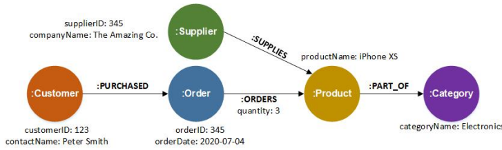
Fig. 3. An example of property graph model.
