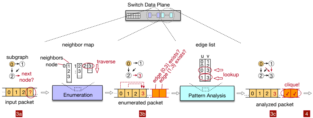
Fig. 5. 3a A packet containing an input subgraph enters the pipeline. 3b The Enumeration process adds/changes edges on the current subgraph using the neighbor map. 3c The Pattern Analysis process checks for potential edges connected to the newly added vertex. 4 If the necessary edges are present, the subgraph contains the desired pattern (e.g., a clique) and is emitted.
