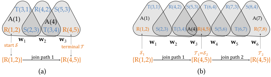
Fig. 1. (a) ILP for triangle query Q_A^\Delta . (b) ILPs are composed by sharing their endpoints (start or terminal tuples).
