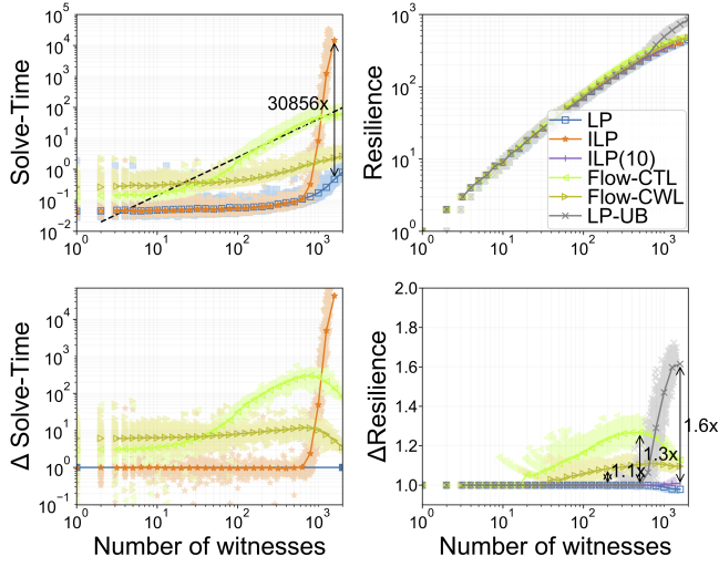
Fig. 5. Setting 1: Hard 3-star query Q_3^\star .
