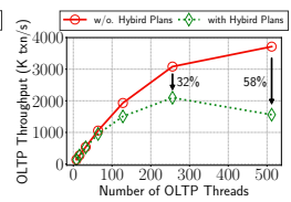
Fig. 4. Freshness Loss Fig. 5. Throughput Drop
