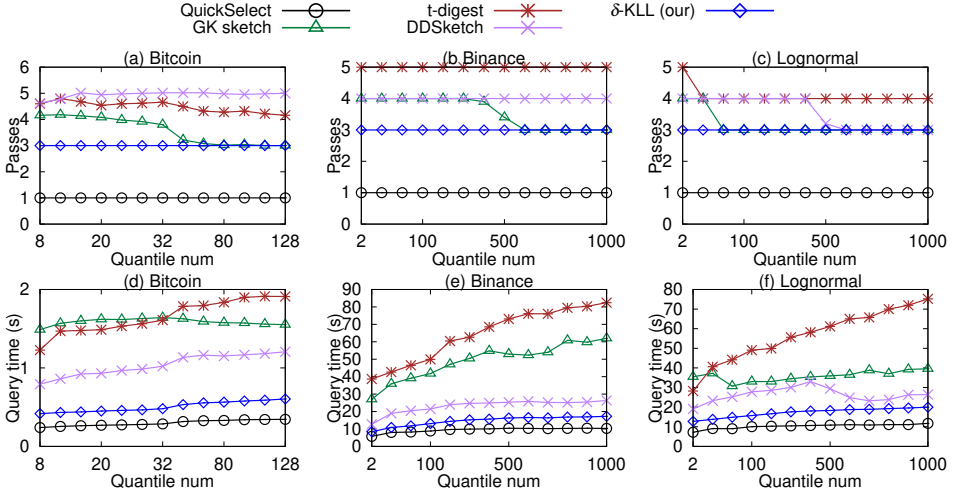
Fig. 19. Allocating K times memory for K quantiles
