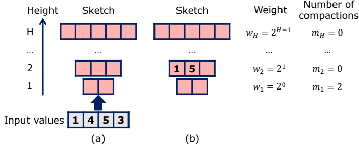
Fig. 3. A sketch with leveled compactors
