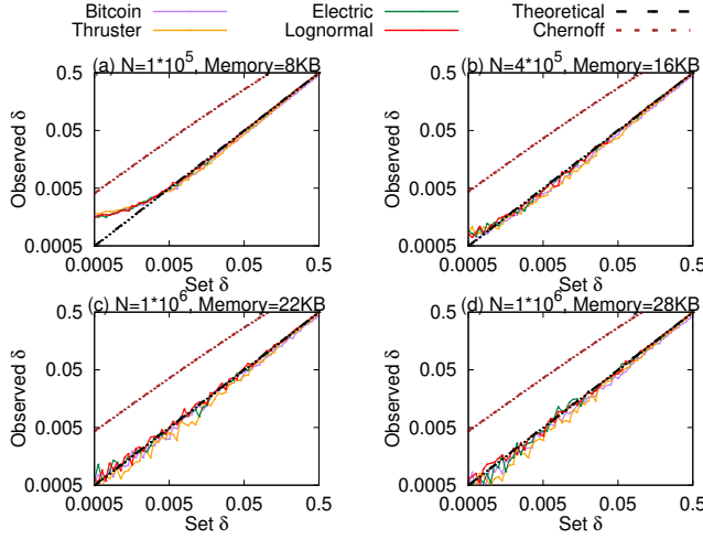
Fig. 13. Accurate failure probability in Formula 3
