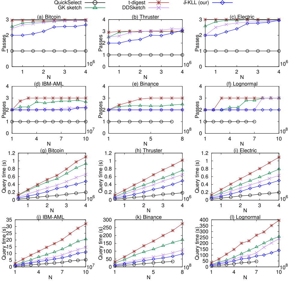
Fig. 16. Varying data size, without pre-computed statistics
