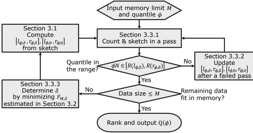
Fig. 5. Quantile query processing
