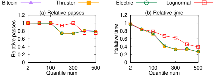
Fig. 22. Relative performance of selecting multiple quantiles with shared pass, compared to no shared pass
