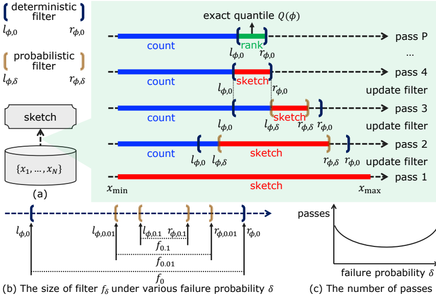
Fig. 2. Our proposal with more aggressive probabilistic filter determined by randomized sketch
