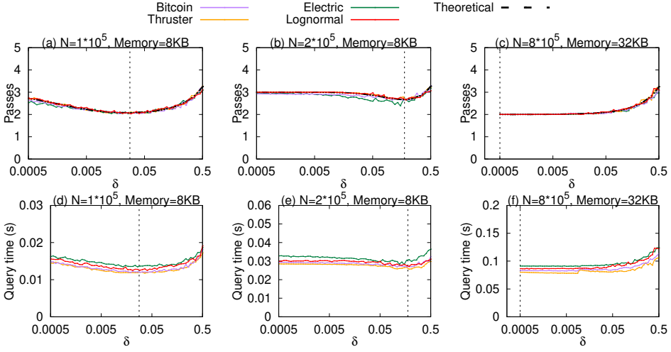
Fig. 14. Accurate pass estimation in Section 3.2
