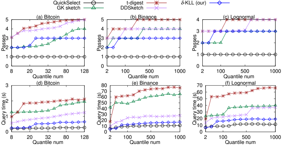
Fig. 18. Comparison by varying number of quantiles
