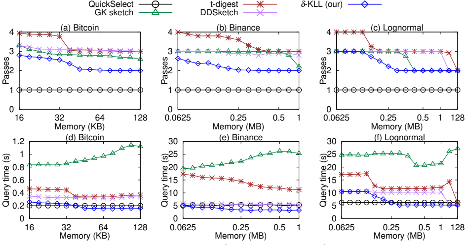
Fig. 17. Comparison by varying memory limit
