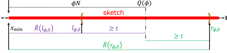
Fig. 6. Probabilistic filter computed in Formula 3
