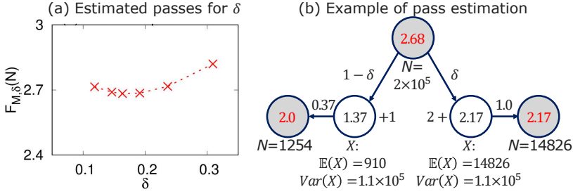
Fig. 8. (a) Estimated passes of some evaluated \delta and (b) Recursive pass estimation for \delta=0.174 in Example 3.6
