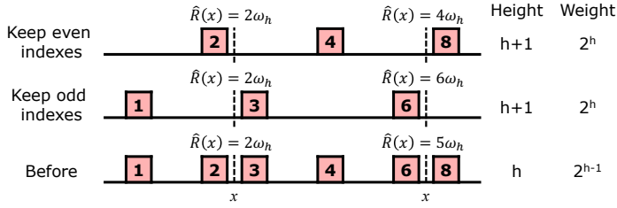
Fig. 4. Influence of randomized compaction
