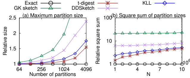
Fig. 23. Relative performances of approximate/exact quantiles in data partition applications for (a) parallel computing and (b) histogram sort
