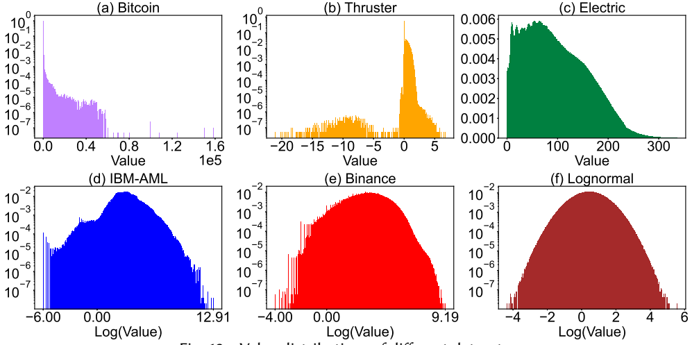
Fig. 12. Value distributions of different datasets
