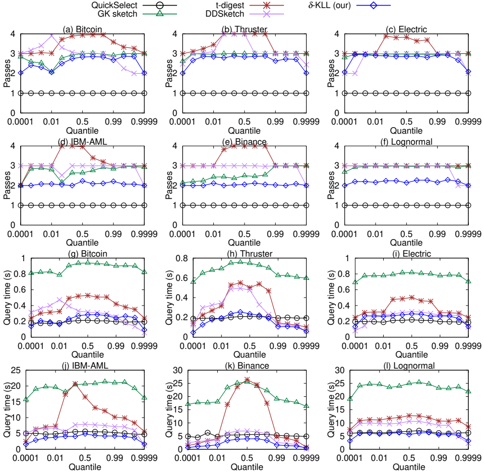
Fig. 20. Comparison by varying queried quantile
