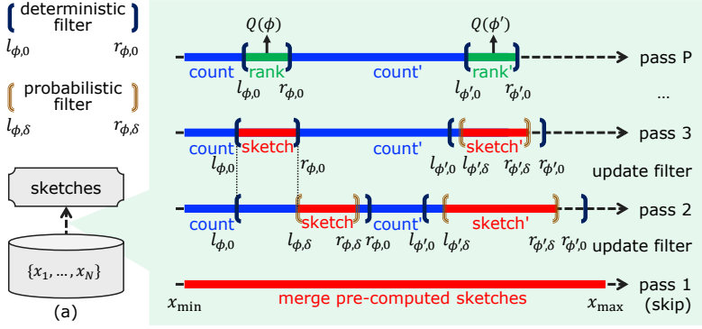
Fig. 10. Computing multiple quantiles
