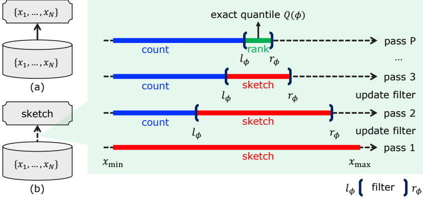
Fig. 1. Existing methods of (a) loading the entire data and (b) multi-pass selection with deterministic sketch
