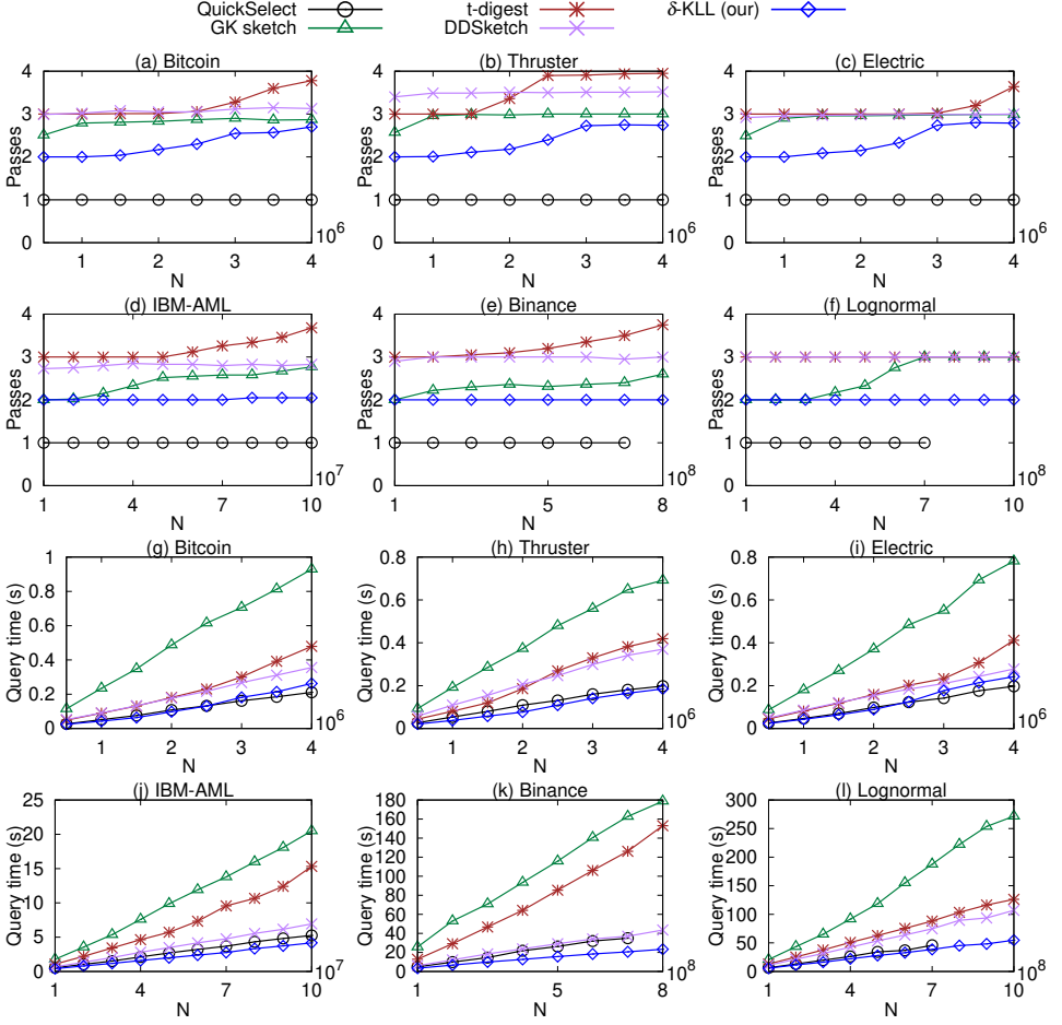
Fig. 15. Comparison by varying data size
