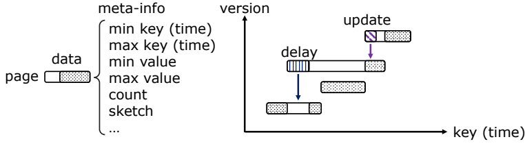
Fig. 11. Pages in LSM-tree store with pre-computed info
