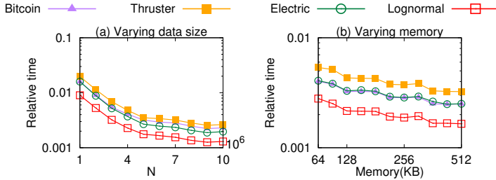
Fig. 21. Relative time cost of determining failure probability \delta , compared to the total time cost of query
