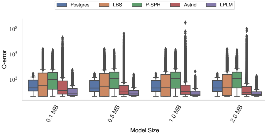
Fig. 5. Q-error of all methods varying space budget.
