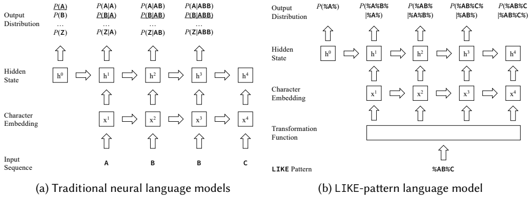
Fig. 2. Probability distribution in traditional and advanced neural language model.
