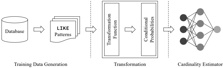
Fig. 3. Summary of our LPLM approach.
