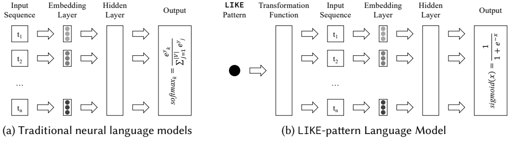
Fig. 1. Comparison of a traditional to our LIKE-pattern Language Model architecture.
