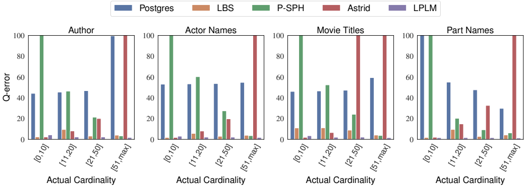
Fig. 4. Geometric mean of Q-errors of different methods for LIKE-patterns varying actual result cardinality.
