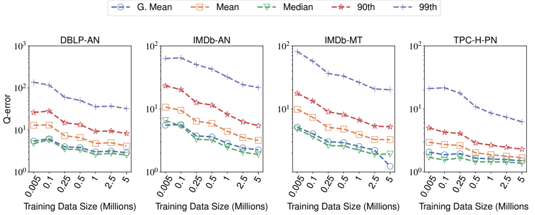
Fig. 6. Geometric mean of Q-errors of LPLM for different sizes of training data set.
