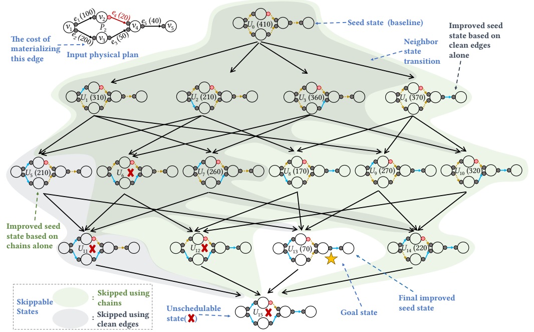
Figure 12. The search process of a simple workflow when running the top-down search Algorithm 1.
