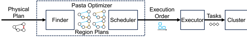
Figure 3. Overview of our proposed Pasta optimizer in a data-processing system.
