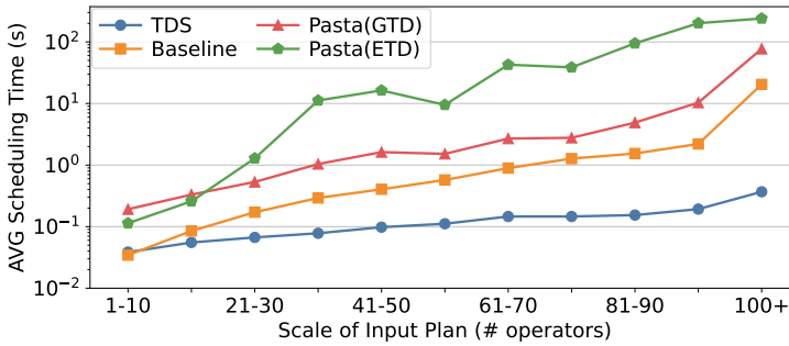
Figure 20. Given a physical plan, the average time it took to generate an execution order for different methods across varying workflow scales.
