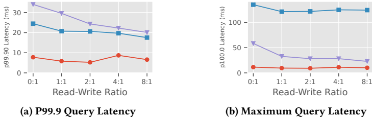
Fig. 16. Tail latency of 3M write queries against a 16 GB Redis database varying read-write ratios (Queue Depth=1000, Payload Size=1 KB, Key Pattern=Gaussian) after snapshot.
