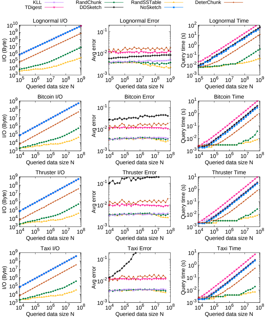
Fig. 11. Performance of memory-constrained solutions with varied N , to provide a guarantee of 0.005 average error if possible, within 2,664 bytes memory except the no-sketch solution
