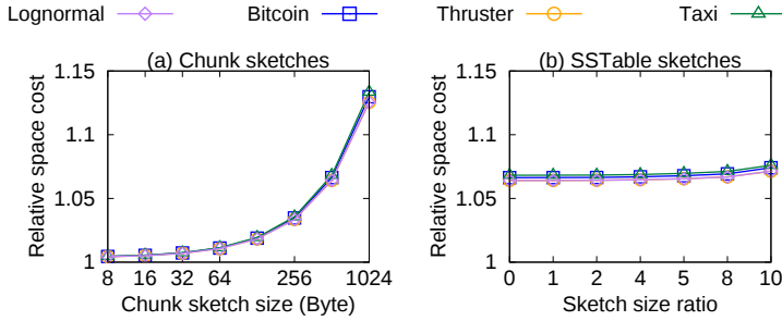
Fig. 13. Space amplification by pre-computed sketches, under (a) various chunk sketch size M_c and (b) various SSTable sketch size ratio T_s , relative to no pre-computation
