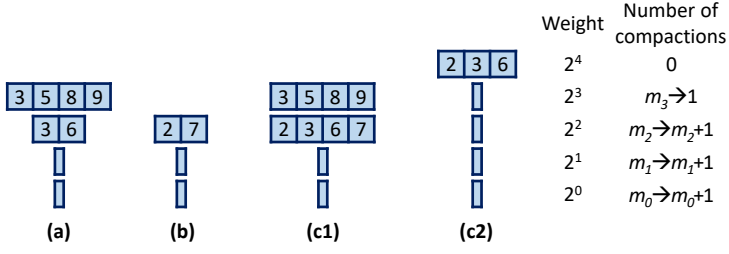
Fig. 6. Process of merging (a) the size-limited KLL sketch S in memory with (b) a pre-computed chunk sketch S_i , resulting in (c2) the merge result after compaction.
