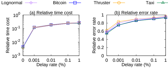
Fig. 15. Query performance improved by pre-computed sketches over the time-series data with various delay rates, relative to no pre-computation
