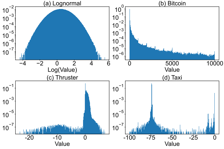
Fig. 9. Value distributions of employed datasets
