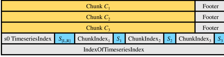
Fig. 7. Storing chunk sketches S_i and SSTable sketches S_{[L,R]} in TsFile
