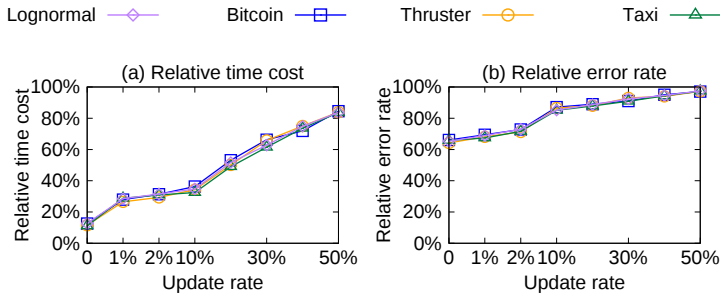
Fig. 16. Query performance improved by pre-computed sketches over the data with various update rates, relative to no pre-computation
