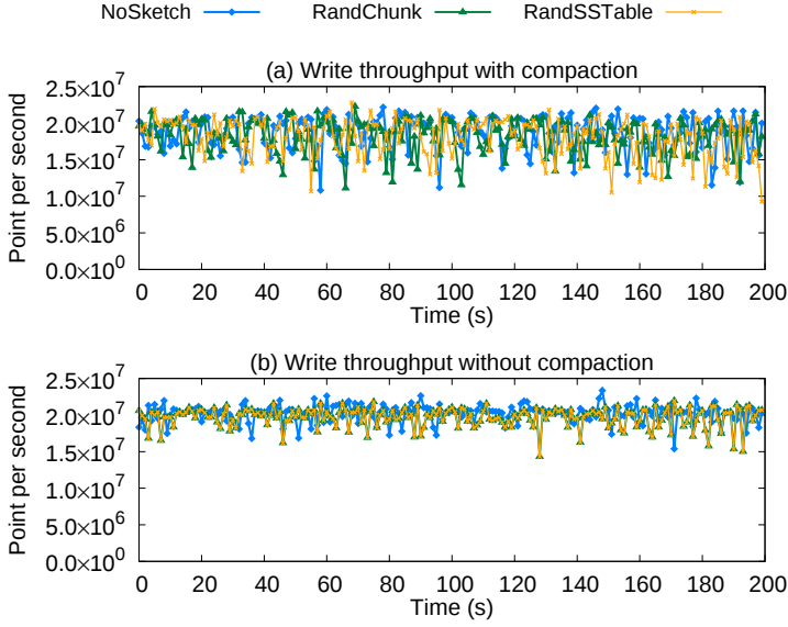
Fig. 14. Write throughput as time, (a) with compactions and (b) without compactions in the scenario
