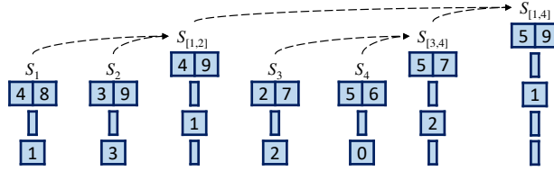
Fig. 5. Example of building hierarchical sketches for a level 2 SSTable with 4 chunks when T = 2 , T_s = 1 . Sketches are organized as an implicit segment tree. S_{[1,4]} is built by combining and further compacting S_{[1,2]} and S_{[3,4]} .
