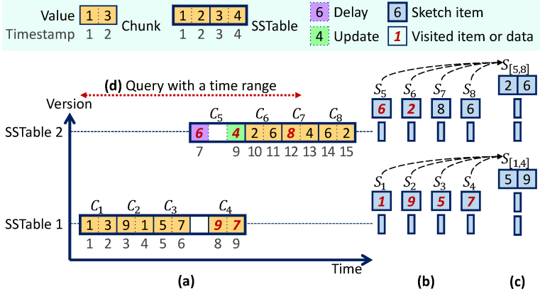
Fig. 8. Solution deployed in Apache IoTDB, with (a) key-range overlapping SSTables caused by delay or update, (b) chunk sketches, (c) SSTable sketches and (d) query posed over data in a time range
