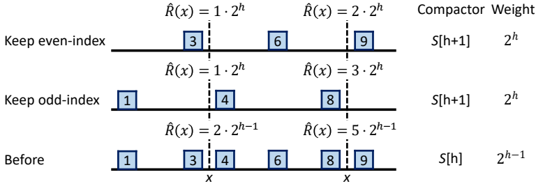
Fig. 3. A randomized compaction over 6 items at height h .
