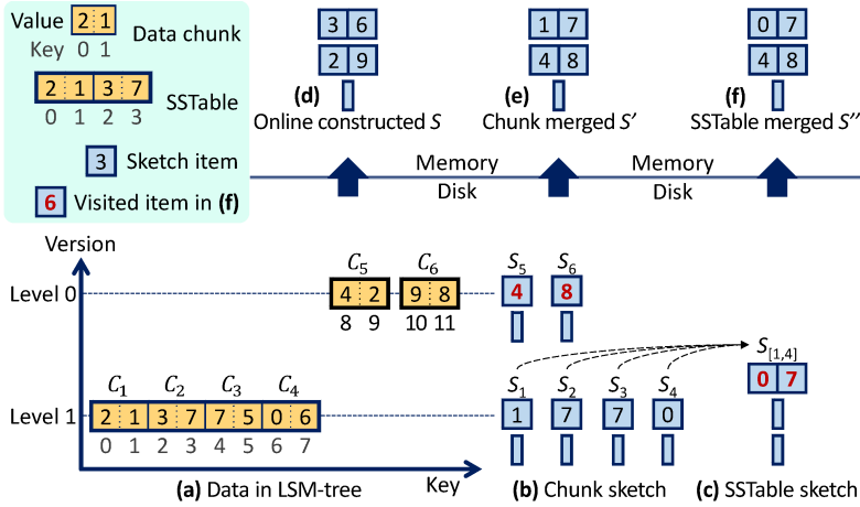
Fig. 1. Overview of quantile estimation on values in LSM-tree based KV store with pre-computed sketches, including (a) data in LSM-based KV store, (b) sketches for chunks in Section 3.1, (c) hierarchical sketches for SSTables in Section 3.2, (d) query processor summarizing data online with a sketch in memory, (e)(f) query processor summarizing pre-computed sketches in Section 4.
