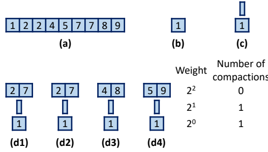
Fig. 4. Example of building a randomized sketch for a chunk with 9 values \{1, 9, 5, 2, 7, 2, 8, 4, 7\} under size limit of 3. (a) sorts all values in memory and (b)(c)(d) assign compactors from bottom to top. (d1)...(d4) show all possible results because of the internal randomness.
