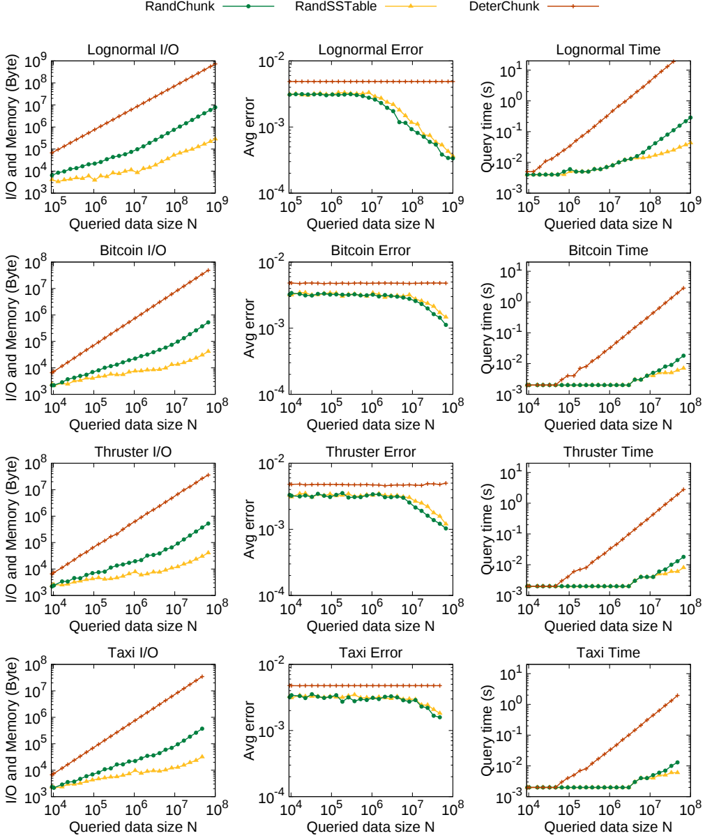
Fig. 10. Performance of disk-bounded solutions with varied N , to provide a guarantee of 0.005 average error
