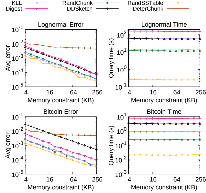
Fig. 12. Varying memory constraint
