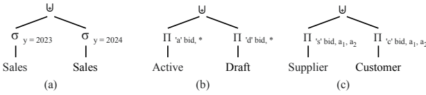
Figure 11: Union All Patterns in S/4HANA
