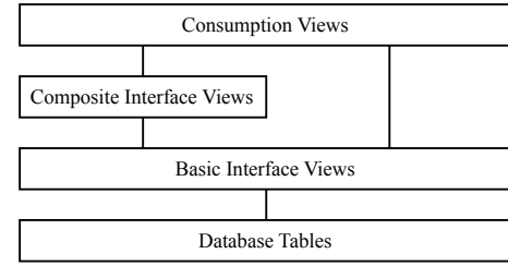
Figure 2: Virtual Data Model Layers
