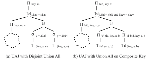
Figure 12: Unused Augmentation Join with Union All
