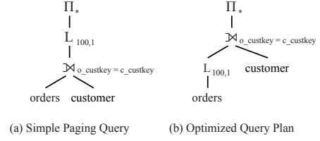
Figure 6: Limit on Augmentation Join
