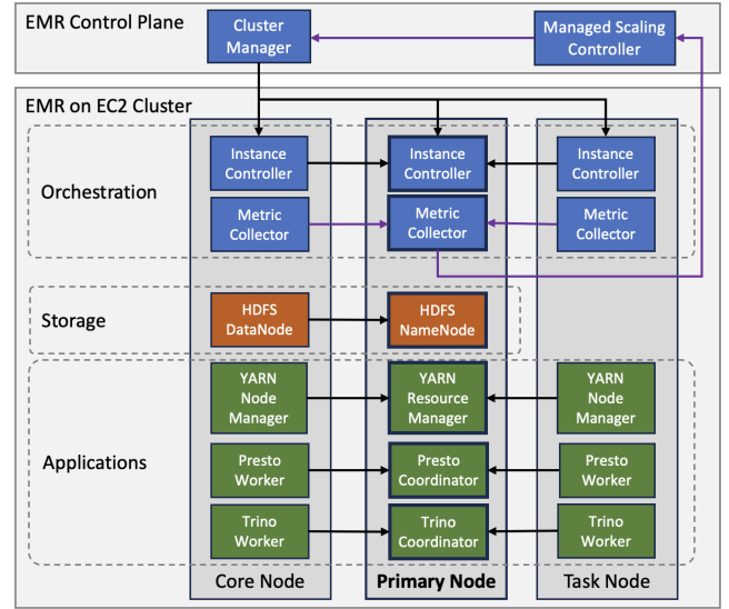
Figure 2: The node types in an EMR-EC2 cluster and how our managed scaling component functions: Instance Controller agents on each node listen to the control plane and perform up-keep of node’s software components. Task Nodes (shown in the right column) only execute tasks and can host workers from any of the application running in the cluster. Core Nodes (in the left column) execute tasks and participate in data storage. The Primary Node (in the middle) hosts the coordinators for all installed applications and collects metrics from the other nodes, forwarding them to the EMS Controller.
