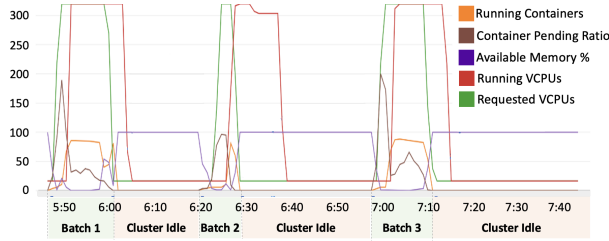
Figure 8: A closer look at EMSv1, when configured to scale a cluster from 1 to 20 nodes, see §6.1.2.
