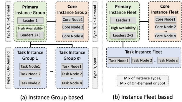
Figure 5: Physical Cluster Topology. Instance Groups (a) consist of homogeneous collections of nodes of the same instance type, lifecycle and availability zones. Instance Fleets (b) mirror a Logical Topology and are characterized by heterogeneity, allowing more flexibility in node choices.
