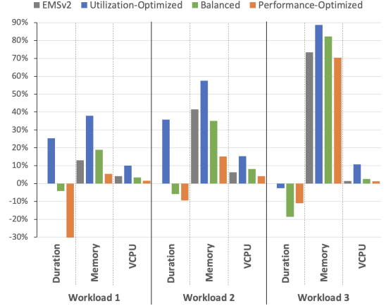
Figure 11: Comparing the three scaling bias presets from §5.3 with the default EMSv2 behavior on three types of workloads; see §6.4.
