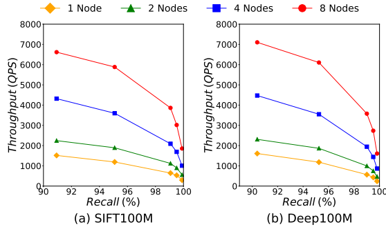
Figure 9: Node Scalability
