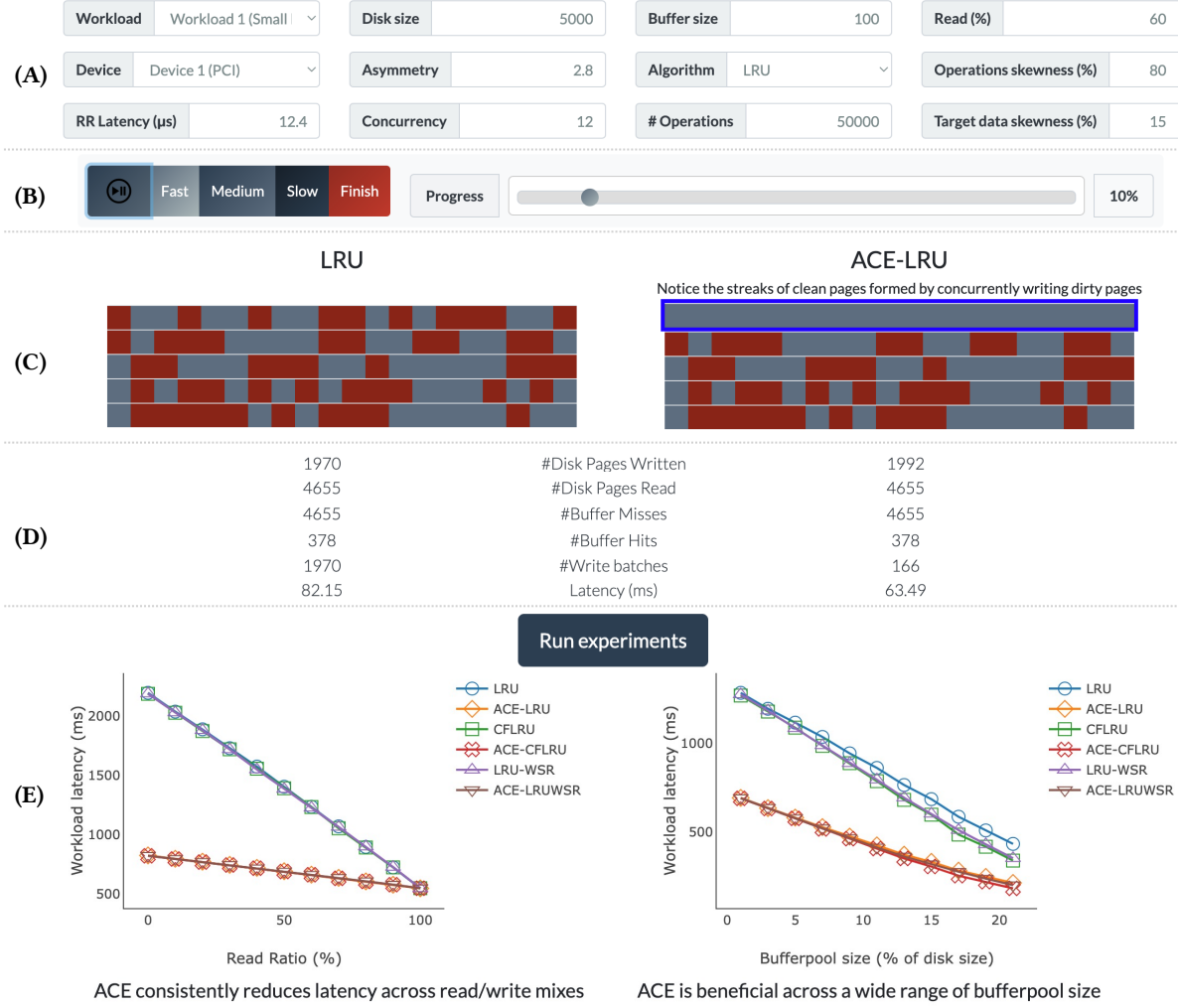
Figure 2: The ACE demonstration UI allows the participants to (A) input workload, disk and bufferpool parameters, (B) control speed and track progress of the simulation, (C) visualize the bufferpool page evictions and writeback along with how ACE creates streak of clean pages due to concurrent writing, (D) compare the performance metrics of the algorithm and its ACE implementation, and (E) run experiments while varying read/write ratio and bufferpool size to analyze ACE’s impact.
