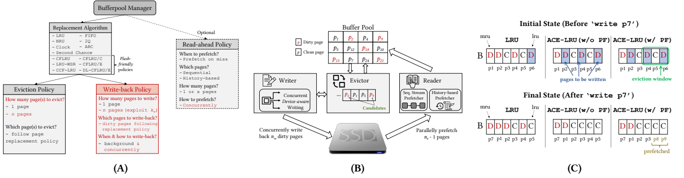
Figure 1: (A) The augmented bufferpool design space (RED denotes new components). (B) Abstract overview of ACE components. (C) Workflow of LRU and ACE-LRU with and without prefetching, when n_w = n_e = 3 .
