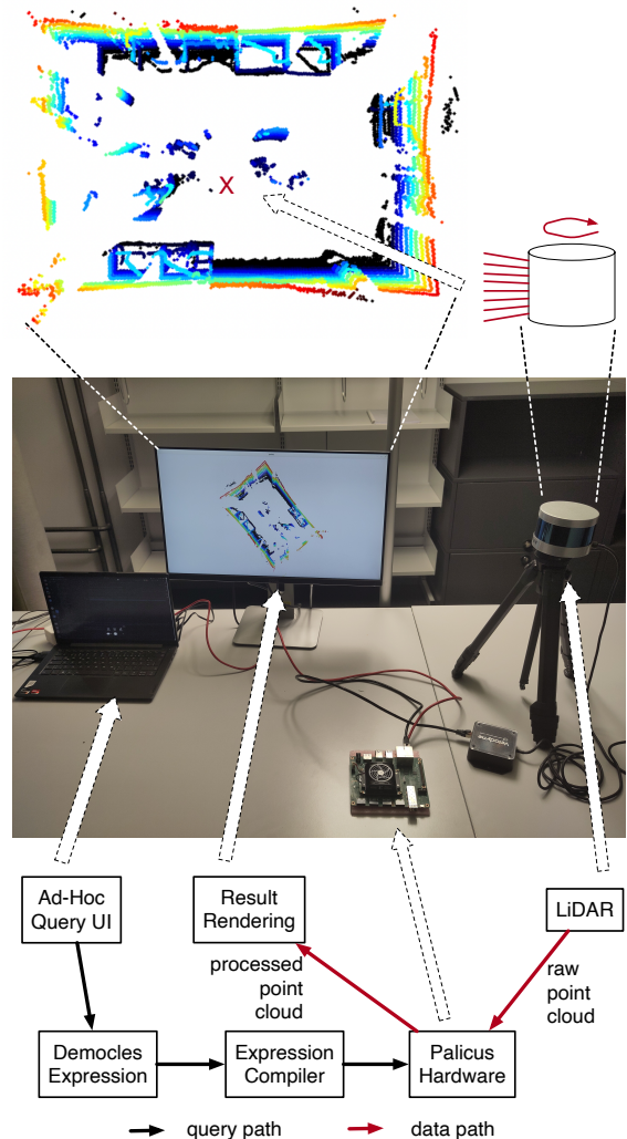
Figure 1: (top) Rendition of Sophie's office point cloud. (center) Demonstration setup: We provide a LiDAR sensor, a PALICUS prototype, and a running instance of ALPHA for data visualization and hardware configuration. (bottom) High-level view of ALPHA: The user writes queries in an intuitive way, which are then emitted as DAMOCLES expressions executed by the programmable hardware.
