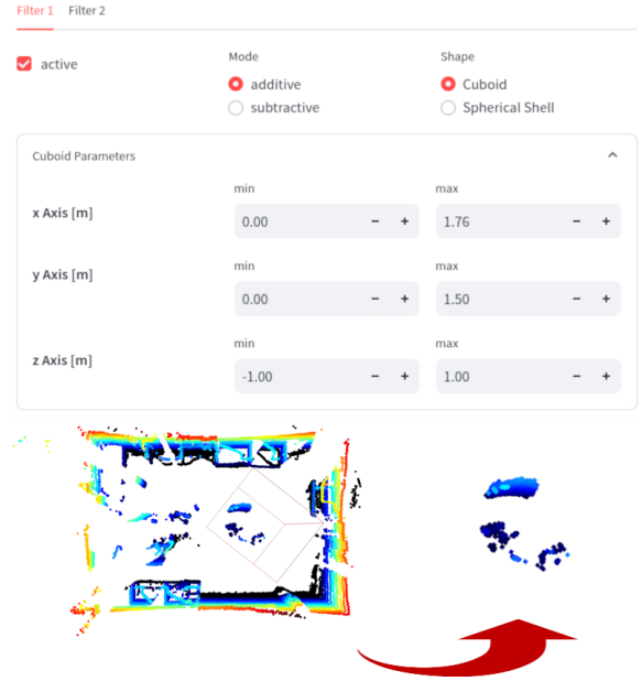
Figure 2: (top) Query-by-example form to express a simple region of interest. (bottom) The effect of applying a cuboid RoI filter on the raw point cloud is seen immediately, including if objects move in or out of the RoI.
