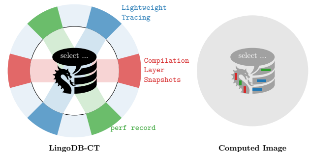
Figure 1: Like computed tomography, LingoDB-CT collects information from different angles about the compilation and execution of a query. Later, this information is correlated to form a more comprehensive picture.
