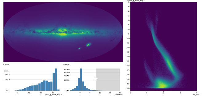
Figure 6: Linked visualizations of over 1.8B stars in the Gaia star catalog. High parallax stars are selected.
