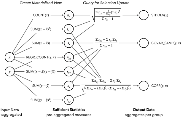
Figure 3: Pre-aggregation and querying for standard deviation and bivariate measures. Each sufficient statistic is included as a column in a materialized view, alongside grouping dimensions. The symbol \hat{x} indicates the average value of x across the full dataset; it is included to mean-center the data to prevent floating point error.
