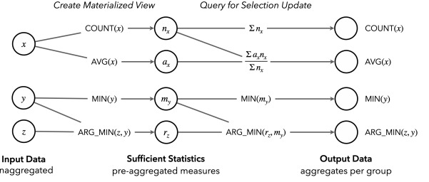
Figure 2: Pre-aggregation and querying for univariate measures. Each sufficient statistic is included as a column in a materialized view, alongside grouping dimensions.
