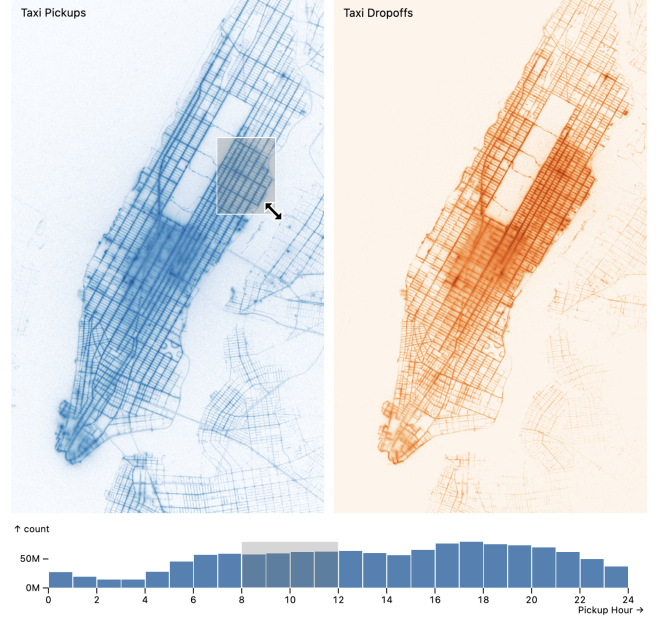
Figure 5: Interactive maps of 1.3B taxi pick-ups and drop-offs in New York City, cross-filtered by pickup time and location.
