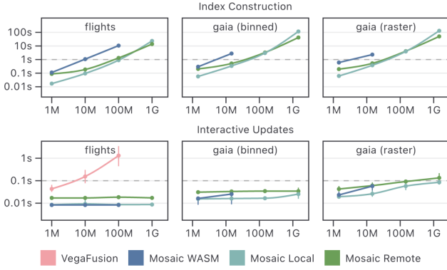
Figure 4: Pre-aggregated materialized view construction (top) and interactive update performance (bottom), from [10]. Median times and interquartile ranges are shown.
