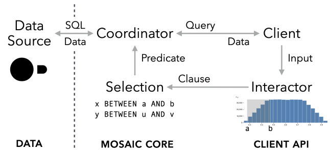
Figure 1: Mosaic architecture overview. A coordinator proxies queries to a backing data source for one or more data-consuming client views. Selections broadcast reactive updates for query predicates. Interactions that update selections may be handled directly by a client, or via interactor components.
