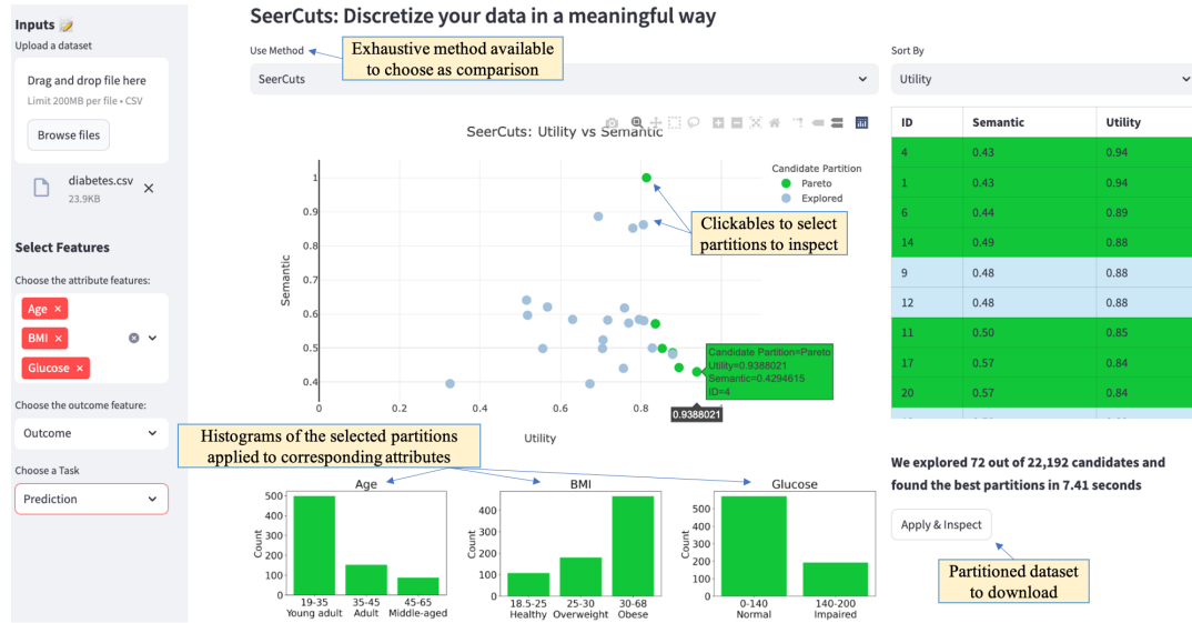
Figure 2: UI of SEERCUTS (example usability for comprehensive modeling).
