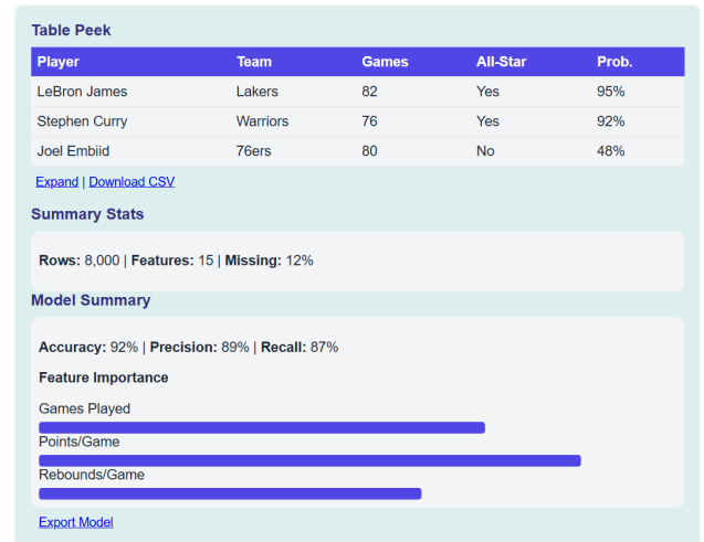
Figure 4: Results Dashboard
