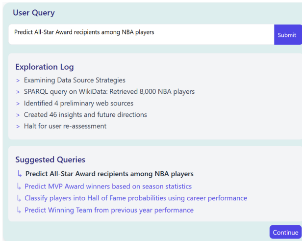
Figure 3: User Interface
