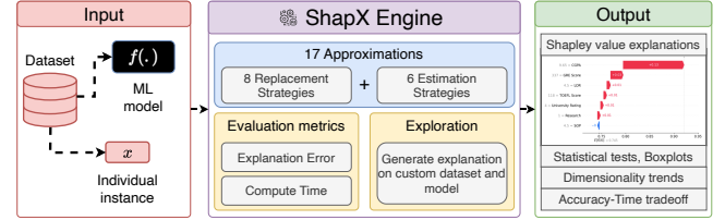
Figure 1: Overview of the Shapley explanation demo system.
