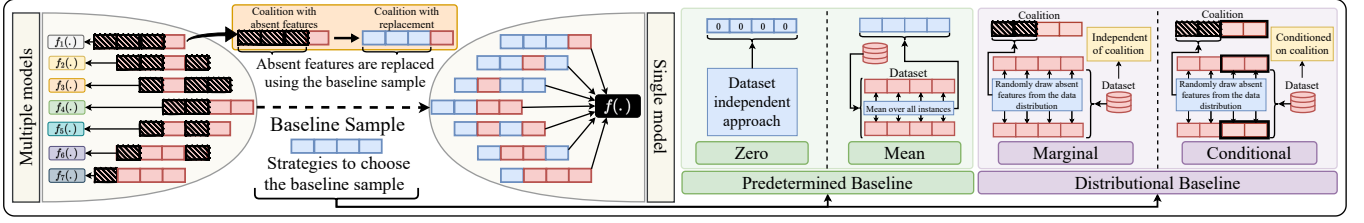
Figure 2: Replacement strategies such as Predetermined Baseline and Distributional Baseline address the absence of features, eliminating the necessity to train an exponential number of models and mitigating computational complexity.
