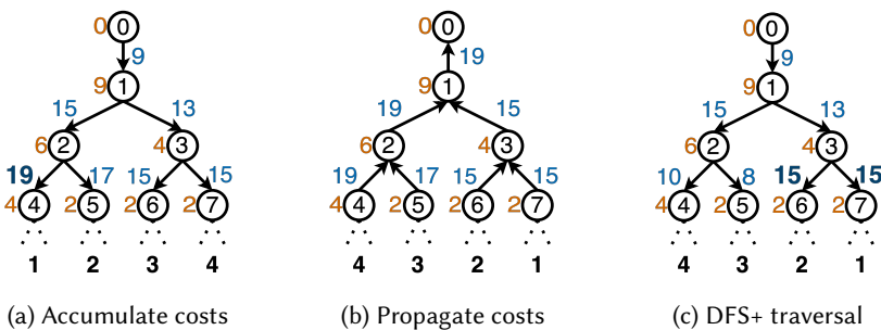
Fig. 9. Example for computing minimum cache requirements to determine a child traversal order for DFS+ : (a) accumulate size of the cache used to traverse a path from the root to a node using a top-down traversal, (b) determine the minimum cache requirement for each subtree as the maximum cache size in the subtree; (c) adjust the minimum cache requirements of edges ending in a node v whose parent has the highest cache requirement among all its siblings by removing the storage size of the parent from all edges below v . Intermediate storage costs are shown in orange, the calculated costs in blue, the maximum is marked in bold, and the traversal order is shown in black below the paths.
