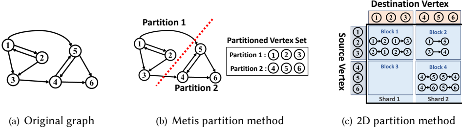
Fig. 3. Graph partition.
