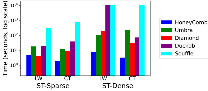
Fig. 12. Performance on Tensor Dataset
