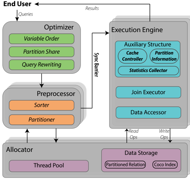
Fig. 5. The Architecture of HoneyComb
