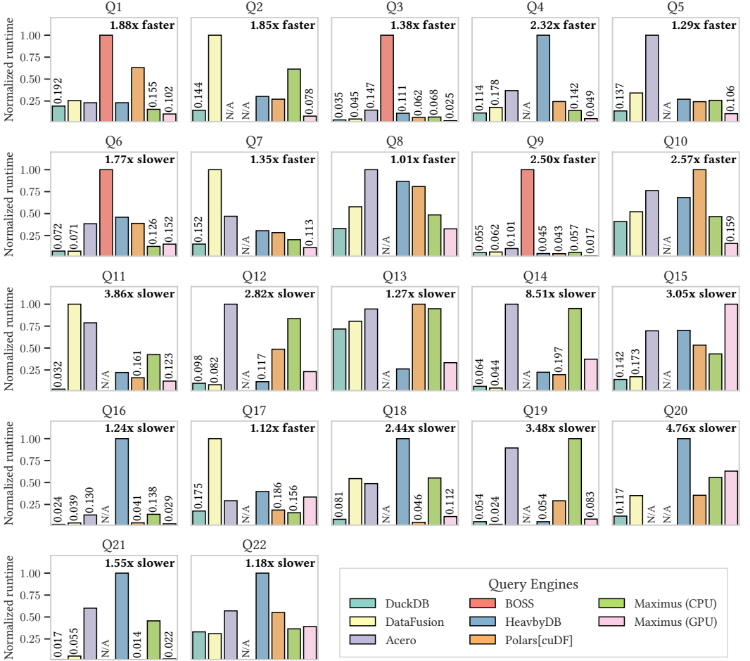
Fig. 8. The execution times for all TPC-H queries for different query engines. All queries start and end on the CPU and all runtimes include all CPU↔GPU data transfer times. The runtimes are normalized by the maximum time for each query. To improve visibility, additional annotations have been added to bars with low height. The upper right corner in each subplot shows the speedup of the best Maximus time (CPU, GPU) vs. the best of other engines.
