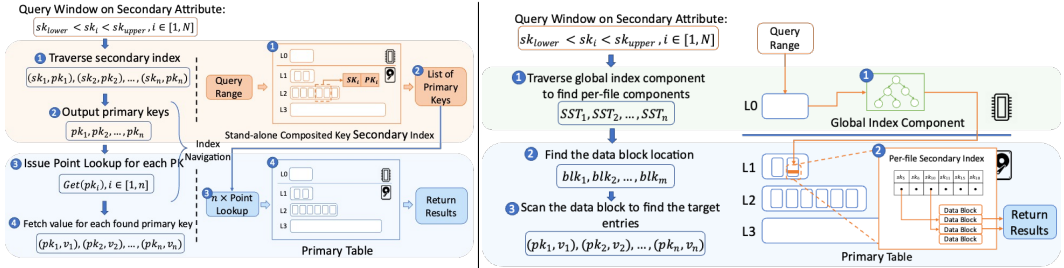
(a) Standalone Secondary Index (b) NEXT secondary index framework Fig. 2. LSM-based Secondary Index Query Processing
