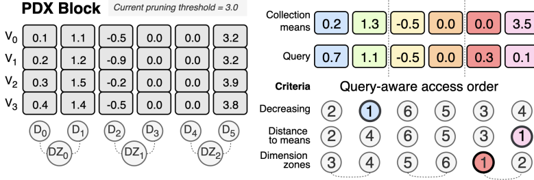
Fig. 5. Example of three query-aware access order criteria: i) Decreasing: the dimension with the highest query value is accessed first ( D_1 in the figure), ii) Distance to means: the dimension of the query with the largest distance to the collection means is accessed first ( D_5 ), iii) Dimension zones: the subset of consecutive dimensions with the highest distance to the collection means are accessed first ( DZ_2 in the figure).
