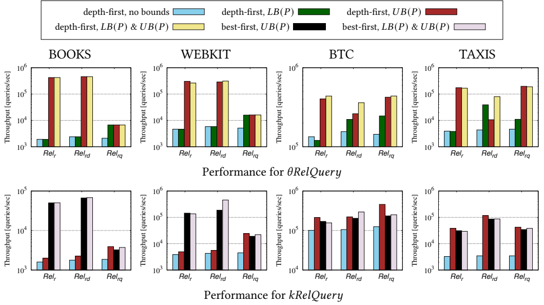
Fig. 9. Query processing on the interval tree; defaults, 0.1% query interval extent, \theta = 0.5 , k = 10
