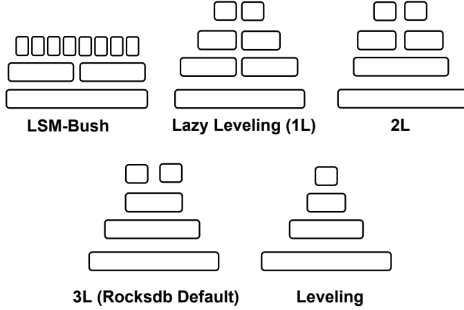
Fig. 2. An overview of different compaction policies.
