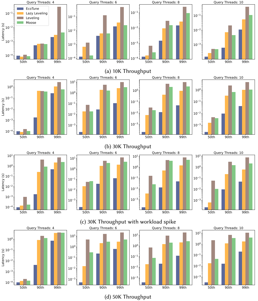
Fig. 9. Latency under different query arrival speeds.
