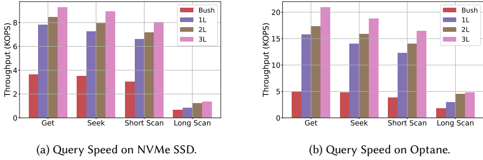
Fig. 3. Speeds of Different Queries. xL means the last x levels are leveling levels.
