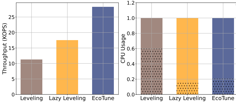
Fig. 1. Average throughput and compaction overhead of different compaction policies. The shadow part corresponds to the compaction's CPU usage.
