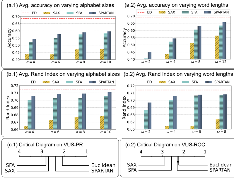
Fig. 12. Comparison between symbolic representations and ED on raw time series: (a) classification; (b) clustering; and (c) anomaly detection. In (a) and (b), ED performance is represented by the red dashed line.
