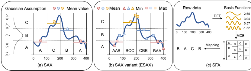
Fig. 1. An overview of symbolic approximation methods. (a) SAX, a classical symbolic method. (b) An example of SAX variant method (ESAX). (c) SFA, a frequency-based method.
