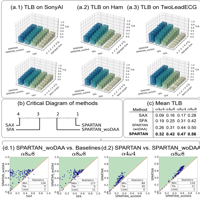
Fig. 7. Evaluation study on TLB, including (a) three representative datasets with varying parameters; (b) critical diagram of SPARTAN and baseline methods; (c) mean TLB value across all 128 UCR datasets under varying parameters; (d) pairwise comparison of SPARTAN_woDAA vs. baselines, and SPARTAN vs. SPARTAN_woDAA.
