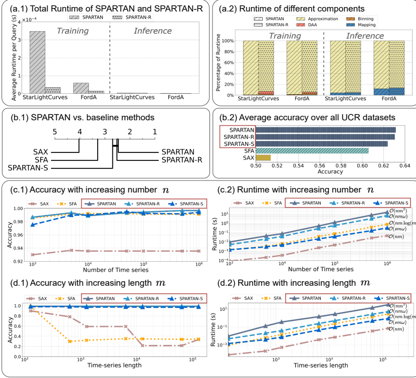
Fig. 10. Accuracy-to-runtime analysis (on 1NN classification task), including (a) runtime analysis on different components of SPARTAN and SPARTAN-R; (b) comparison of SPARTAN methods vs. SAX and SFA on UCR datasets; (c,d) accuracy-to-runtime analysis on large-scale datasets.
