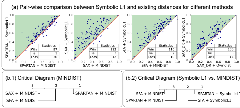
Fig. 11. Ablation study on the symbolic distances (evaluated on 1NN classification task). (a) pair-wise comparison between Symbolic L_1 and existing distance (denoted as MINDIST or “Owndist”); and (b) Average rankings on SPARTAN, SFA, and SAX, over MINDIST and Symbolic L_1 .
