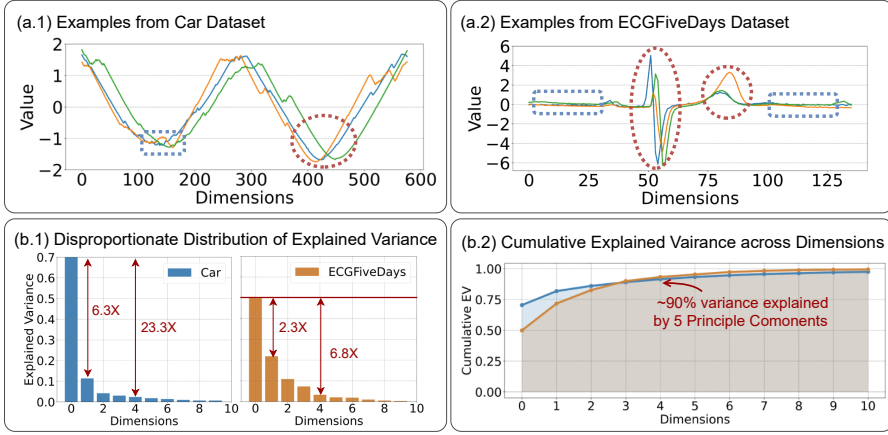
Fig. 3. Measure of informativeness across dimensions on Car and ECGFiveDays datasets: (a) representative examples from each dataset, with flat regions highlighted in blue bounding boxes and representative patterns in red ellipses; and (b) explained variance for the top latent dimensions.
