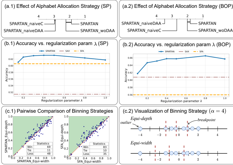
Fig. 6. Ablation study of SPARTAN on 1NN Classification task. (a) Critical diagrams of SPARTAN with different alphabet allocation strategies; (b) Classification accuracy with varying regularization parameter \lambda ; and (c) Comparison of two binning strategies, Equi-depth and Equi-width.
