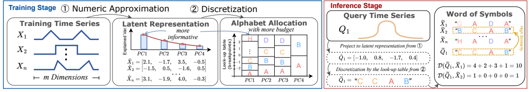
Fig. 2. An overview of SPARTAN pipeline: (a) training stage, including the data-dependent approximation and dynamic discretization; and (b) inference stage, where query samples can be transformed on the fly.
