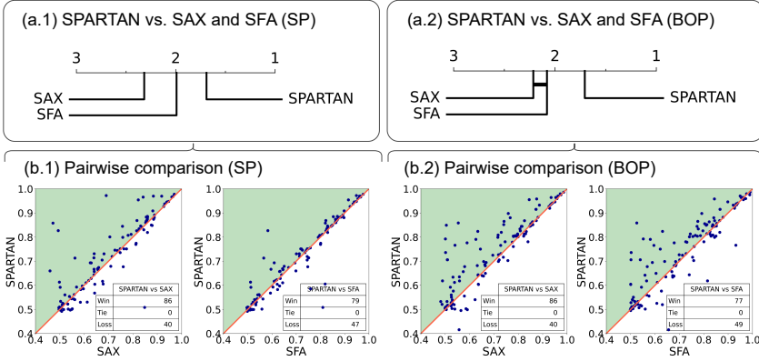
Fig. 8. Evaluation study on the clustering downstream task, including (a) CD plots of SPARTAN and top two baselines; (b) pairwise comparison on UCR datasets.
