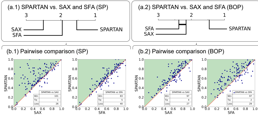
Fig. 5. 1NN Classification evaluation of SPARTAN, SAX and SFA, including (a) critical diagrams with statistical test; (b) pair-wise comparisons on all 128 UCR datasets.
