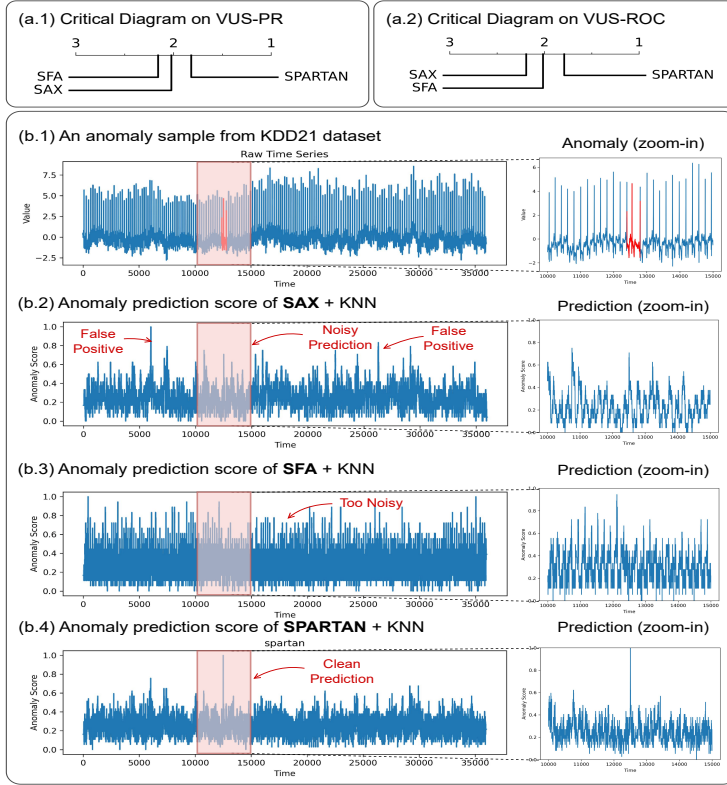
Fig. 9. Anomaly detection evaluation on symbolic methods + KNN detector, including (a) CD plots evaluated by VUS-PR/VUS-ROC; (b) visualization of an anomaly example from KDD21 dataset and the prediction results of each method. The red bounding box and lines highlight the anomalies.
