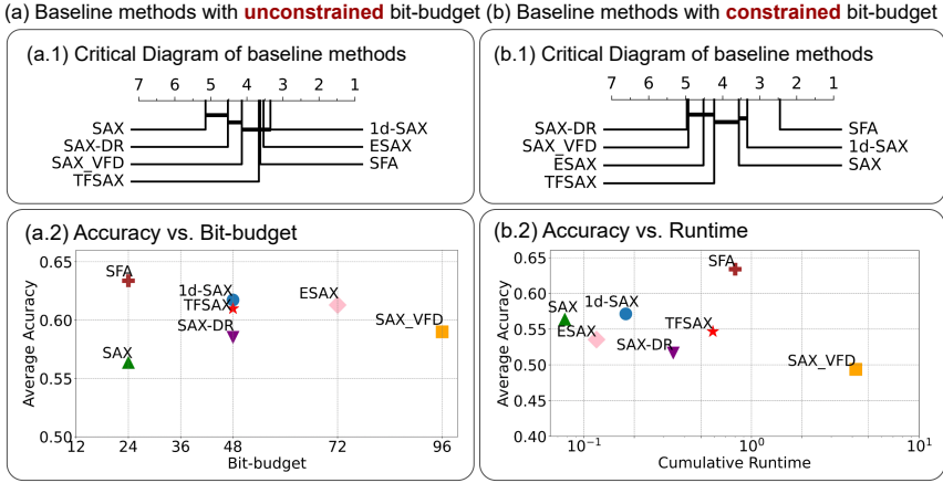
Fig. 4. Evaluation of 7 baseline methods on 1NN classification accuracy, bit-budget, and runtime (in seconds) with (a) unconstrained bit-budget and (b) constrained bit-budget. The solid line in the critical diagram (CD) plots connects all methods that do not perform statistically differently according to the Nemenyi test.
