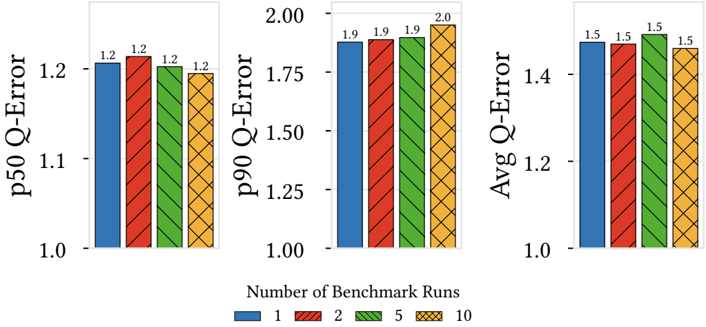
Fig. 14. Model accuracy for different number of benchmark runs. There is no evidence that multiple benchmark runs improve model performance significantly.
