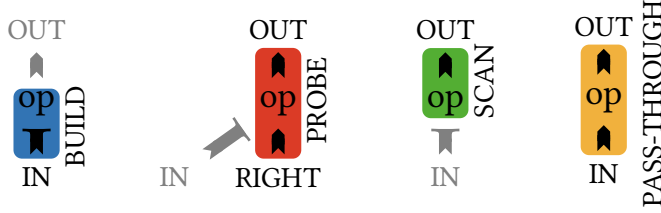
Fig. 4. Operators can have multiple stages: build, probe, scan, and pass-through. Furthermore, each operator has up to three tuple streams for data input (IN, RIGHT) or output (OUT). At each end we can consider basic features of the pipeline.
