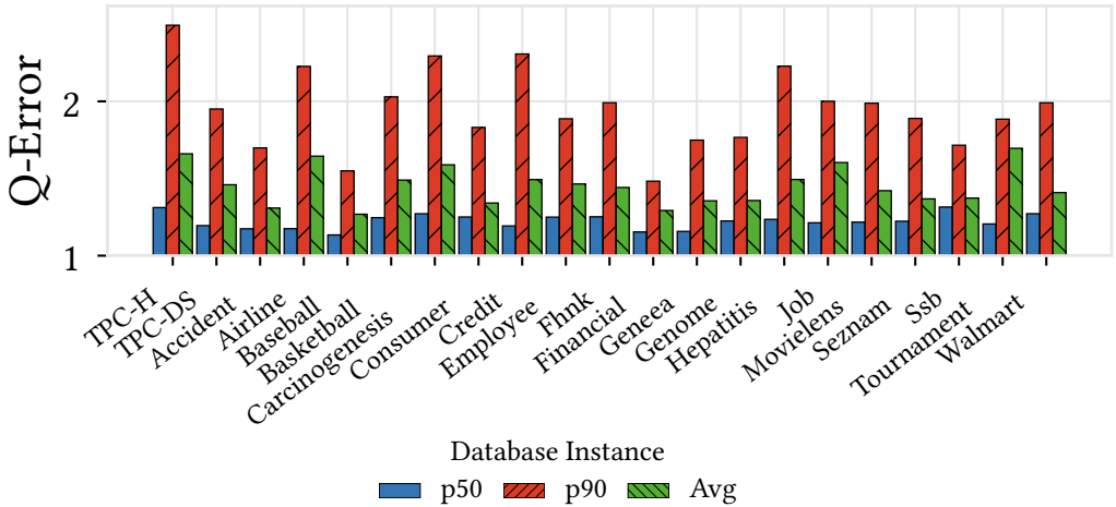
Fig. 9. Different q-errors for different evaluation database instances. T3 is always trained on all but one database instance and then evaluated on the left-out instance. For TPC-H and TPC-DS, the respective numbers include different scale factors.
