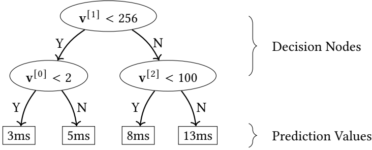
Fig. 3. Example of a two level decision tree. During evaluation, we traverse the decision nodes of the tree. Once we reach a leaf, we return the corresponding prediction value.
