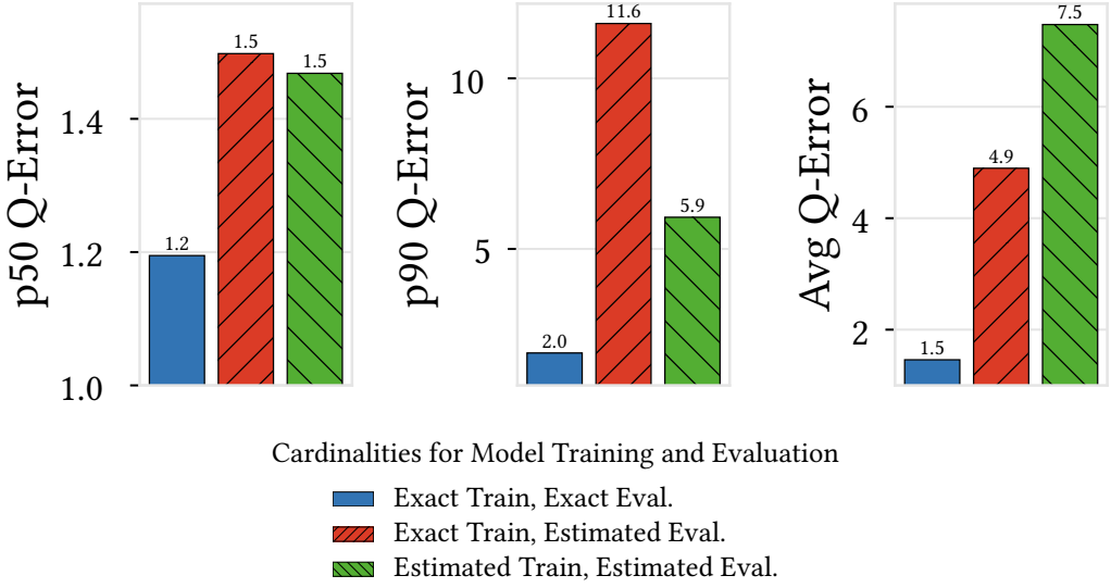
Fig. 11. Accuracy with perfect and estimated cardinalities. Three variants: 1. A model trained on perfect cardinalities and evaluated on perfect cardinalities. 2. Same model trained on perfect cardinalities and evaluated on estimated cardinalities. 3. Model trained on estimated cardinalities and evaluated on estimated cardinalities. Median (p50) q-error left, p90 q-error middle, and avg q-error right. Evaluation on all TPC-DS test queries on scale factors 1, 10, and 100.
