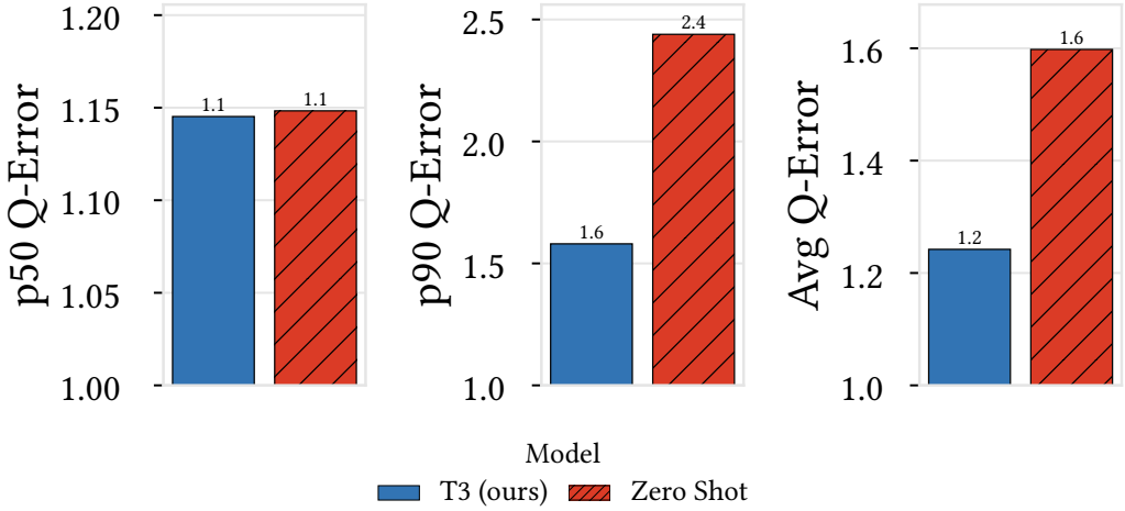
Fig. 10. Accuracy comparison of Zero Shot model and T3. Both are trained on other database instances and evaluated on the queries of the Join Order Benchmark.
