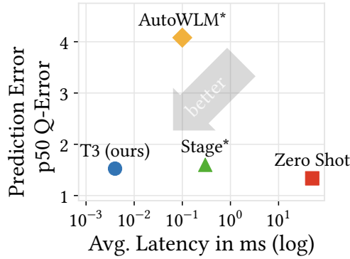
Fig. 1. Latency and accuracy of recent models [16, 40, 50]. (*values from [50])
