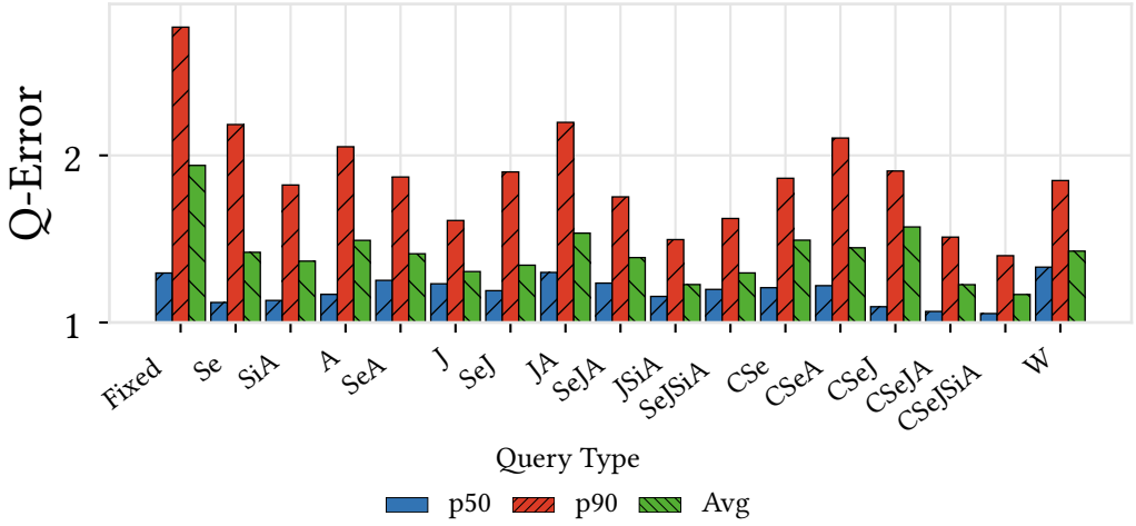
Fig. 8. Different q-errors for different query types on TPC-DS data. Benchmark queries (Fixed) as well as generated queries: Selections (Se), aggregations (A), simple aggregations (SiA), joins (J), complex selections (CSe), window functions (W), and combinations of them.
