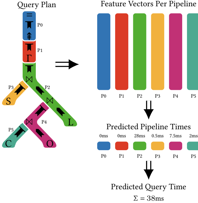
Fig. 2. T3 prediction process for TPC-H Q5. Each pipeline is converted to a flat feature vector. T3’s decision tree model predicts a time for each feature vector. The sum of the predicted pipeline times is the result.
