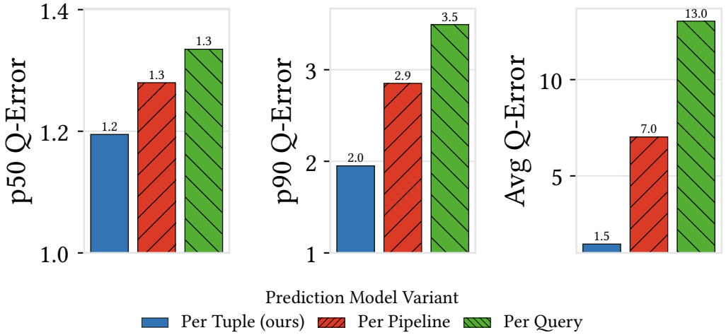
Fig. 13. T3 accuracy when predicting for a single tuple, an individual pipeline, or a whole query. The second variant tries to directly predict the execution time for the whole pipeline. The third variant predicts on a single feature vector that is the sum of all pipeline feature vectors.
