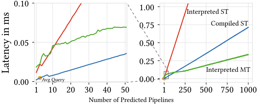
Fig. 5. T3’s prediction latency by number of pipelines. Compiled T3 is always single-threaded (ST), interpretation can also be executed multi-threaded (MT). The average query consists of 3 pipelines and has a prediction latency of 4us.
