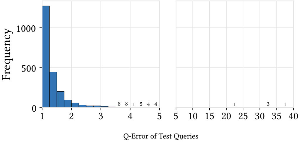
Fig. 7. Frequency distribution of different q-errors for T3 predictions on all TPC-DS test queries.
