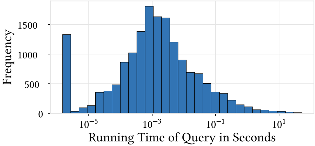
Fig. 6. Observed running times of queries in our dataset.
